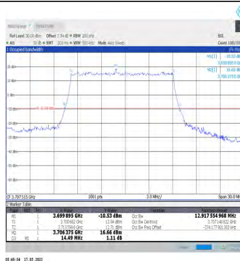
1-N77-3700-3980-30-15-L-1-DFT-QPSK-Outer_Full-36@0-Ant1-12.918-14.490-≤15-PASS
