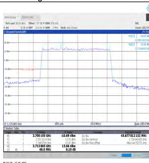
1-N77-3700-3980-30-50-L-3-DFT-16QAM-Outer_Full-128@0-Ant1-45.678-48.000-≤50-PASS
