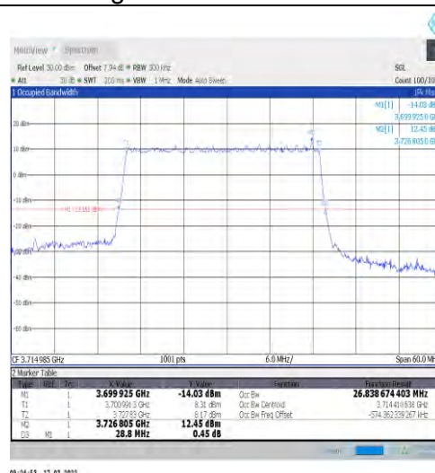
1-N77-3700-3980-30-30-L-5-DFT-256QAM-Outer_F ull-75@0-Ant1-26.839-28.800-≤30-PASS
