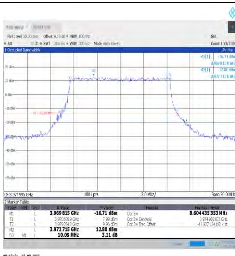
1-N77-3700-3980-30-10-H-7-CP-16QAM-Outer_Full-24@0-Ant1-8.604-10.080-≤10-PASS
