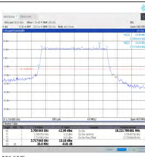
1-N77-3700-3980-30-20-L-7-CP-16QAM-Outer_Full-51@0-Ant1-18.222-20.000-≤20-PASS
