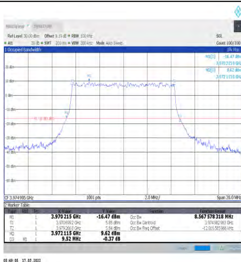
1-N77-3700-3980-30-10-H-9-CP-256QAM-Outer_Full-24@0-Ant1-8.568-9.520-≤10-PASS
