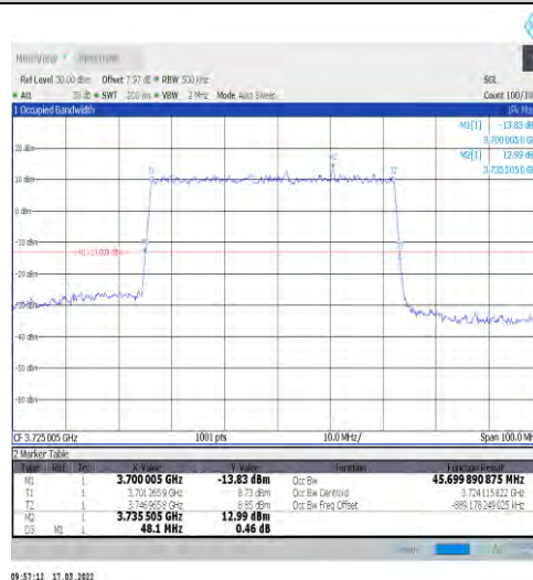
1-N77-3700-3980-30-50-L-5-DFT-256QAM-Outer_Full-128@0-Ant1-45.7-48.100-≤50-PASS
