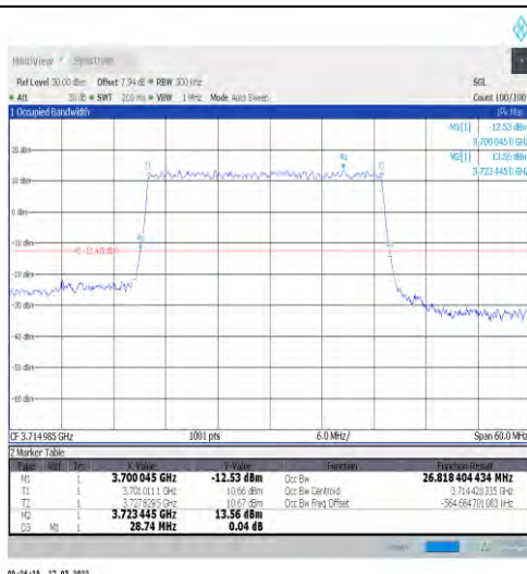
1-N77-3700-3980-30-30-L-4-DFT-64QAM-Outer_Full -75@0-Ant1-26.818-28.740-≤30-PASS
