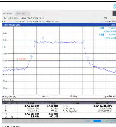
1-N77-3700-3980-30-10-L-9-CP-256QAM-Outer_Full -24@0-Ant1-8.594-9.900-≤10-PASS
