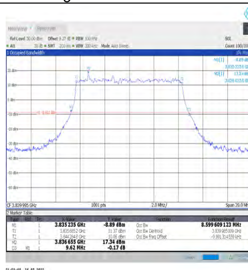
1-N77-3700-3980-30-10-M-1-DFT-QPSK-Outer_Full- 24@0-Ant1-8.6-9.620-≤10-PASS
