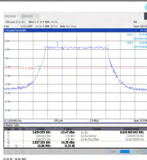
1-N77-3700-3980-30-10-M-3-DFT-16QAM-Outer_Ful l-24@0-Ant1-8.635-10.060-≤10-PASS
