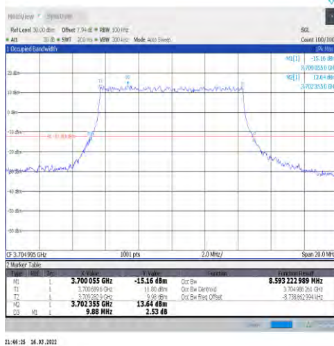
1-N77-3700-3980-30-10-L-3-DFT-16QAM-Outter_Full-24@0-Ant1-8.593-9.880-≤10-PASS
