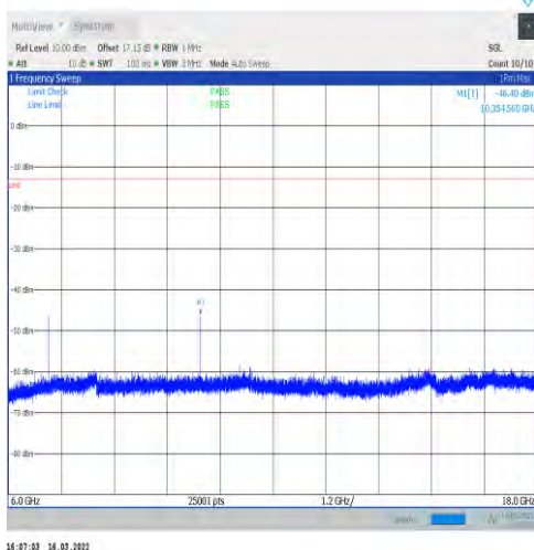
1-N77-3450-3550-30-100-L-1-DFT-PI2BPSK-Inner_1 RB_Left-1@1-6000-18000-Ant1--46.40--13-PASS
