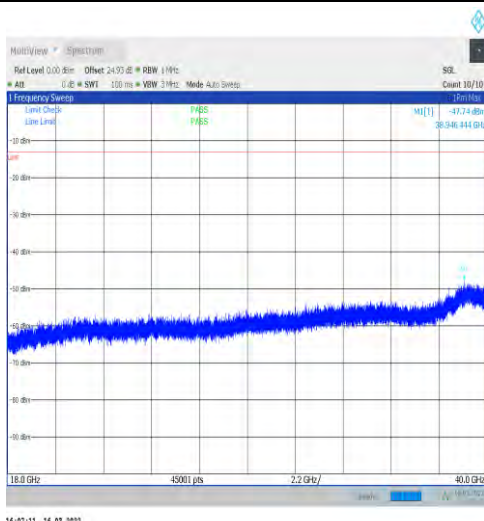
1-N77-3450-3550-30-100-L-1-DFT-PI2BPSK-Inner_1 RB_Left-1@1-18000-40000-Ant1--47.74--13-PASS
