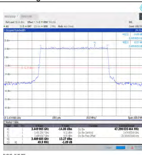
1-N77-3450-3550-30-50-L-7-CP-16QAM-Outter_Full-133@0-Ant1-47.398-49.900-≤50-PASS
