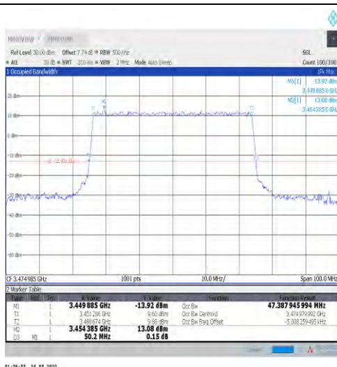
1-N77-3450-3550-30-50-L-6-CP-QPSK-Outter_Full-1 33@0-Ant1-47.388-50.200-≤50-PASS
