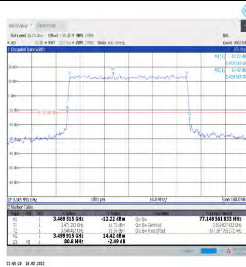
1-N77-3450-3550-30-80-H-4-DFT-64QAM-Outer_Ful I-216@0-Ant1-77.149-80.800-≤80-PASS
