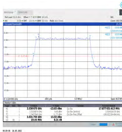
1-N77-3450-3550-30-20-H-4-DFT-64QAM-Outer_Full-50@0-Ant1-17.877-19.440-≤20-PASS
