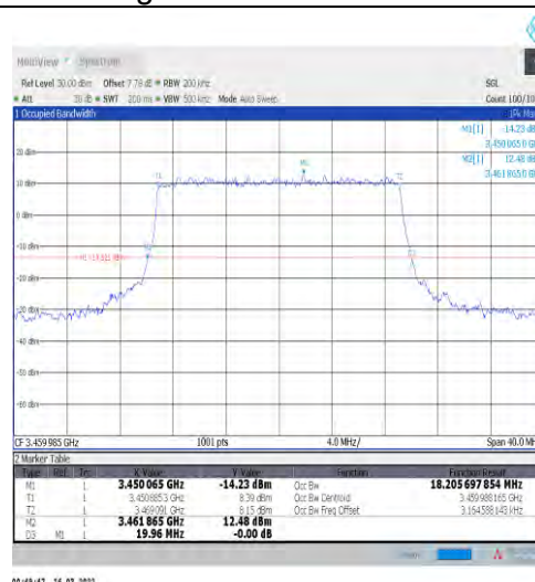
1-N77-3450-3550-30-20-L-8-CP-64QAM-Outer_Full-51@0-Ant1-18.206-19.960-≤20-PASS
