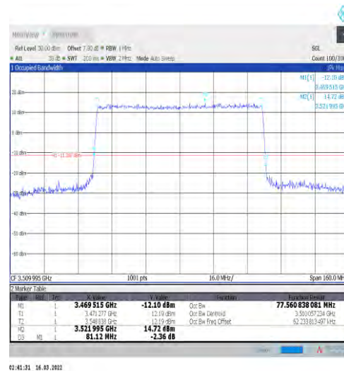
1-N77-3450-3550-30-80-H-6-CP-QPSK-Outer_Full-2 17@0-Ant1-77.561-81.120-≤80-PASS
