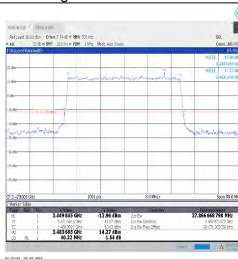
1-N77-3450-3550-30-40-L-6-CP-QPSK-Outer_Full-1 06@0-Ant1-37.867-40.320-≤40-PASS
