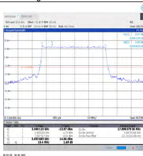
1-N77-3450-3550-30-20-M-3-DFT-16QAM-Outer_Full-50@0-Ant1-17.898-19.400-≤20-PASS
