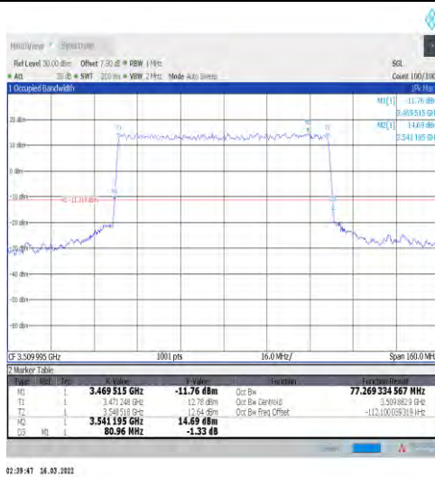
1-N77-3450-3550-30-80-H-3-DFT-16QAM-Outer_Ful I-216@0-Ant1-77.269-80.960-≤80-PASS
