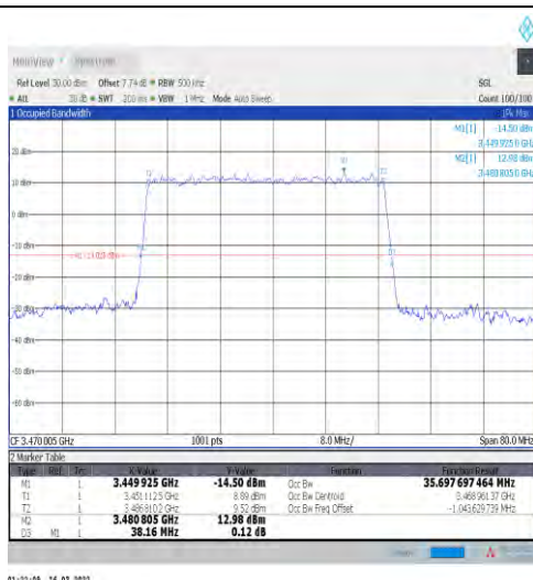
1-N77-3450-3550-30-40-L-5-DFT-256QAM-Outer_Fu II-100@0-Ant1-35.698-38.160-≤40-PASS
