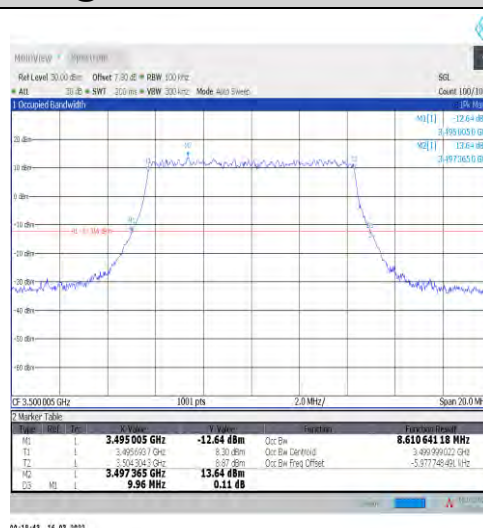
1-N77-3450-3550-30-10-M-3-DFT-16QAM-Outer_Ful I-24@0-Ant1-8.611-9.960-≤10-PASS
