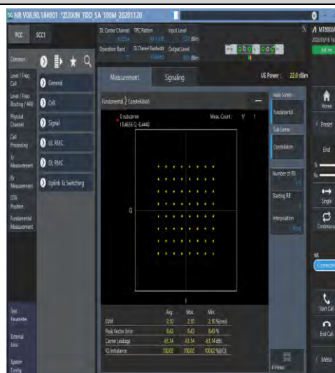
1-N77-3450-3550-30-100-M-8-CP-64QAM-Outer_Full-273@0-Ant1-see graph-PASS
