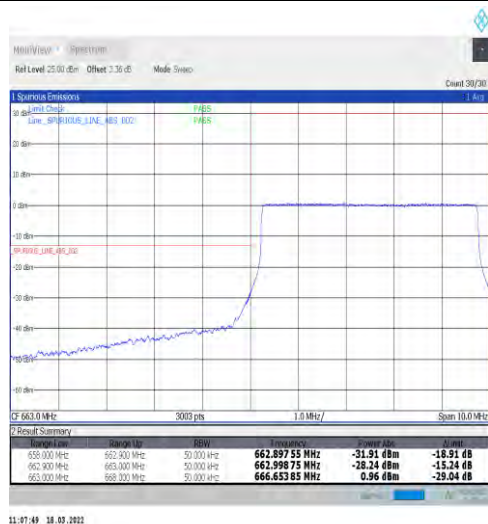
1-N71-15-5-L-6-CP-QPSK-Outer_Full-25@0-Ant1-PASS-see graph
