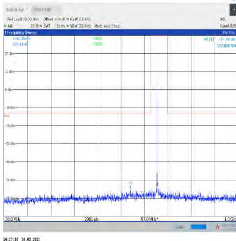
1-N71-15-20-L-1-DFT-PI2BPSK-Inner_1RB_Left-1@ 1-30-1000-Ant1--54.78--13-PASS
