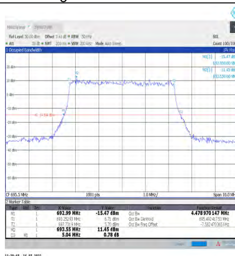
1-N71-15-5-H-4-DFT-64QAM-Outer_Full-25@0-Ant1 -4 479-5 040-≤5-PASS
