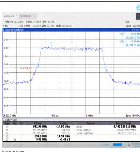
1-N71-15-5-H-3-DFT-16QAM-Outer_Full-25@0-Ant1 -4 463-5 010-<5-PASS
