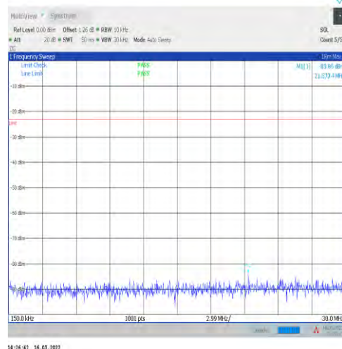
1-N71-15-20-L-1-DFT-PI2BPSK-Inner_1RB_Left-1@ 1-0.15-30-Ant1--83.86--23-PASS
