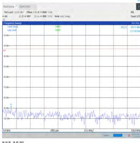
1-N71-15-20-L-1-DFT-PI2BPSK-Inner_1RB_Left-1@ 1-0.009-0.15-Ant1--89.67--33-PASS
