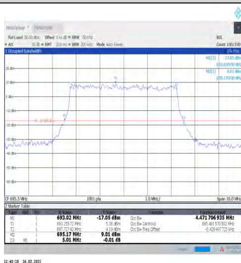
1-N71-15-5-H-5-DFT-256QAM-Outer_Full-25@0-Ant 1-4.472-5.010-≤5-PASS
