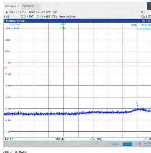
1-N71-15-20-L-1-DFT-PI2BPSK-Inner_1RB_Left-1@ 1-1000-3000-Ant1--48.40--13-PASS
