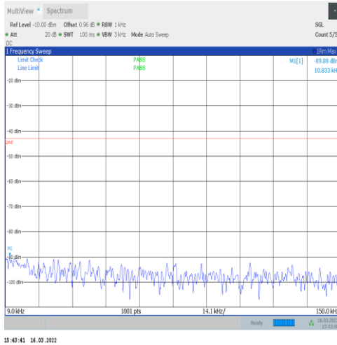
1-N70-15-15-M-1-DFT-PI2BPSK-Inner_1RB_Left-1@ 1-0.009-0.15-Ant1--89.88--43-PASS
