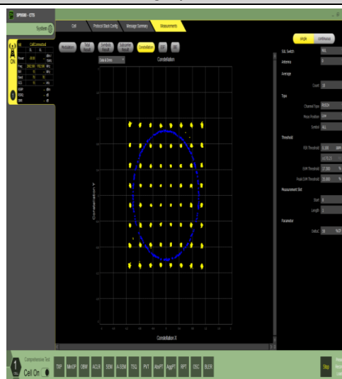
1-N70-15-15-M-4-DFT-64QAM-Outer_Full-75@0-Ant1-see graph-PASS
