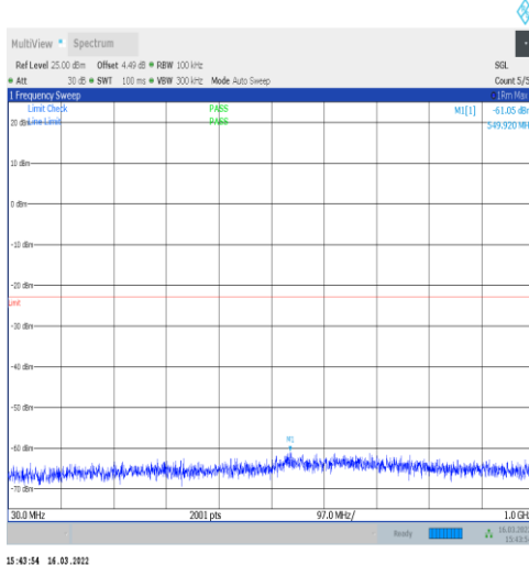
1-N70-15-15-M-1-DFT-PI2BPSK-Inner_1RB_Left-1@ 1-30-1000-Ant1--61.05--23-PASS
