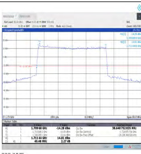
1-N66-15-40-L-6-CP-QPSK-Outer_Full-216@0-Ant1- 38.649-40.480-≤40-PASS
