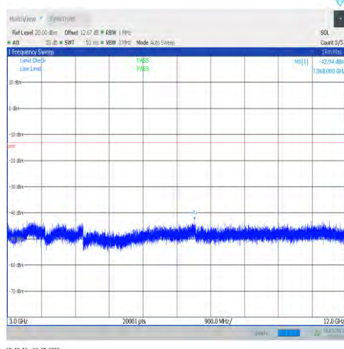
1-N66-15-40-M-1-DFT-PI2BPSK-Inner_1RB_Left-1 @1-3000-12000-Ant1--42.94--13-PASS
