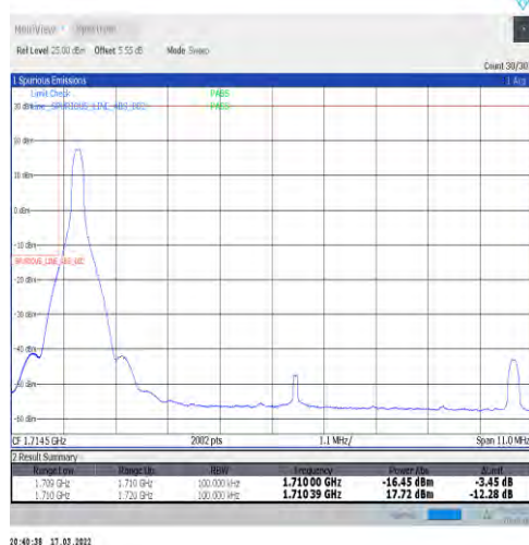
1-N66-15-10-L-4-CP-QPSK-Edge_1RB_Left-1@0-Ant1-seegraph-PASS-see graph
