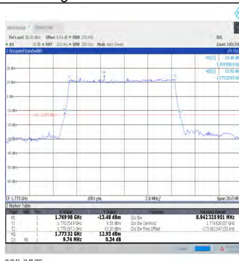
1-N66-15-10-H-1-DFT-QPSK-Outer_Full-50@0-Ant1 -8.942-9.740≤10-PASS
