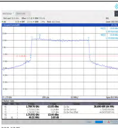
1-N66-15-40-L-8-CP-64QAM-Outer_Full-216@0-Ant 1-38.69-40.320-≤40-PASS
