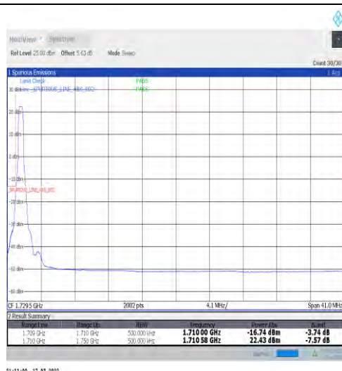
1-N66-15-40-L-1-DFT-PI2BPSK-Edge_1RB_Left-1@0-Ant1-seegraph-PASS-see graph
