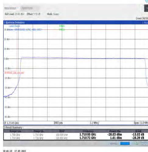
1-N66-15-10-L-6-CP-QPSK-Outer_Full-52@0-Ant1-seegraph-PASS-see graph
