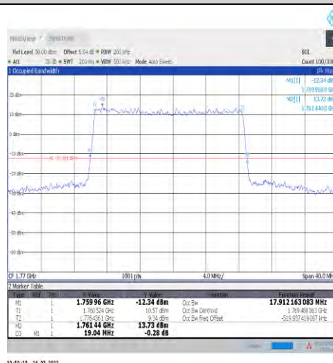
1-N66-15-20-H-1-DFT-QPSK-Outer_Full-100@0-Ant 1-17.912-19.040-≤20-PASS
