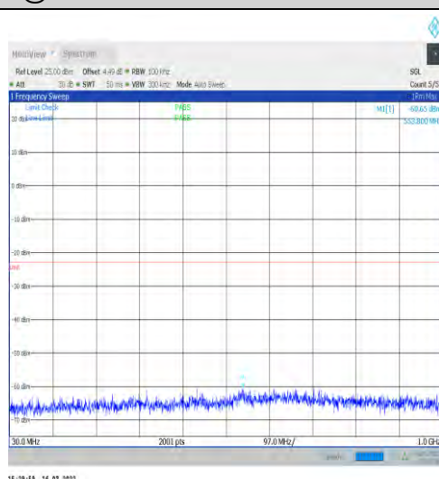
1-N66-15-40-H-1-DFT-PI2BPSK-Inner_1RB_Left-1 @1-30-1000-Ant1--60.65--23-PASS
