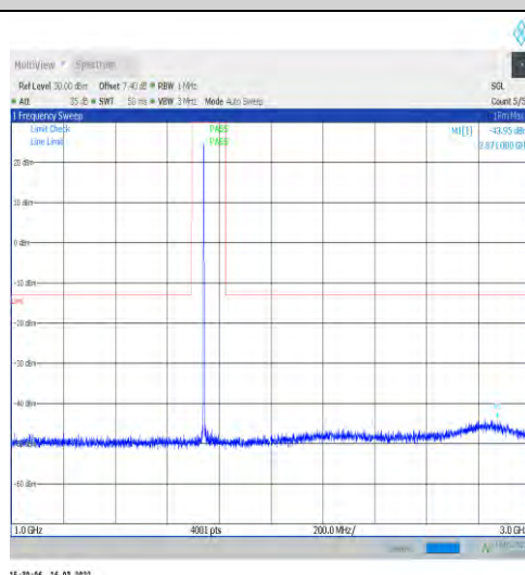
1-N66-15-40-H-1-DFT-PI2BPSK-Inner_1RB_Left-1@ 1-1000-3000-Ant1--43.95--13-PASS
