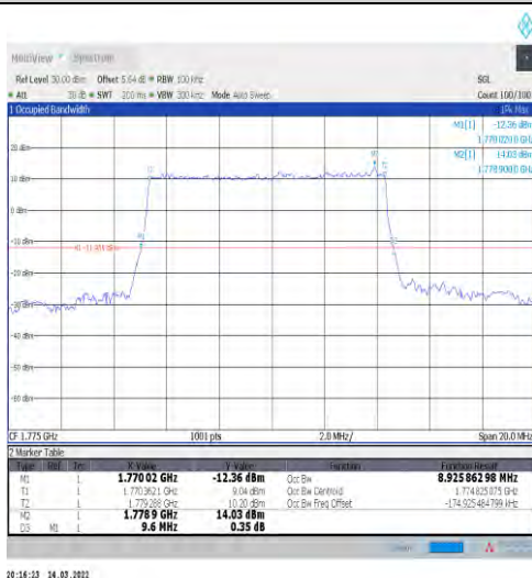
1-N66-15-10-H-2-DFT-PI2BPSK-Outer_Full-50@0-Ant1 nt1-8.926-9.600≤10-PASS
