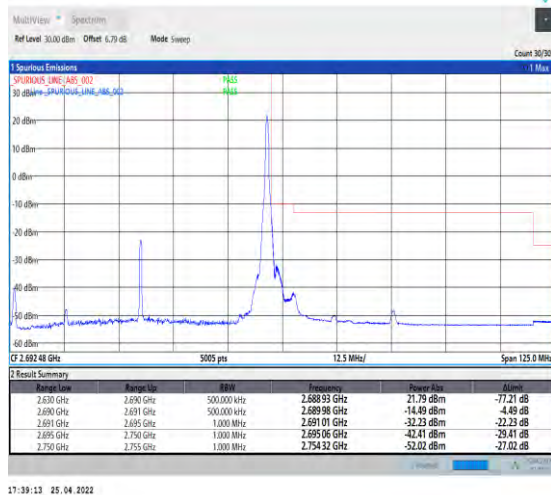
1-N41--30-60-H-5-CP-QPSK-Edge_1RB_Right-1@161-Ant 1-PASS-see graph
