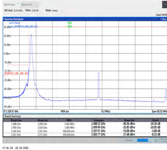
1-N41--30-70-L-4-CP-QPSK-Edge_1RB_Left-1@0-Ant 1-PASS-see graph
