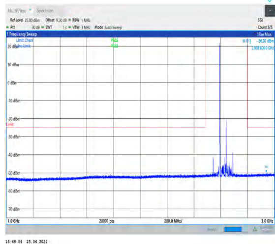
1-N41--30-100-H-1-DFT-QPSK-Edge_1RB_Left-1@ -1000-3000-Ant1--50.07--25-PASS
