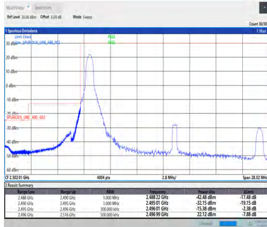
1-N41--30-20-L-4-CP-QPSK-Edge_1RB_Left-1@0-Ant 2-PASS-see graph
