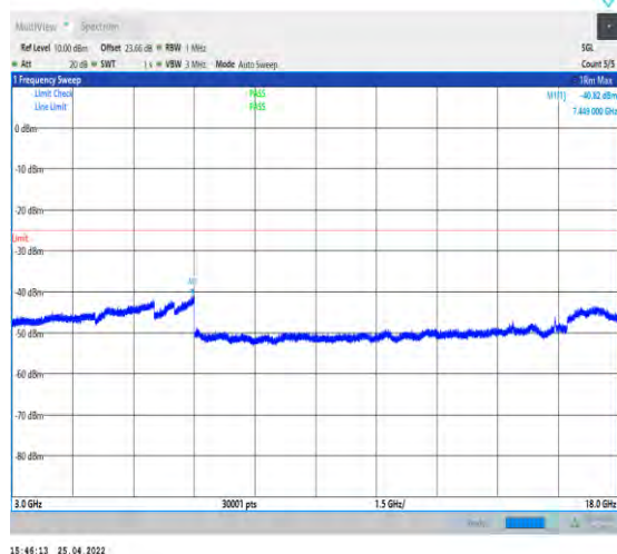
1-N41--30-100-L-1-DFT-QPSK-Edge_1RB_Left-1@ 0-3000-18000-Ant1--40.82--25-PASS
