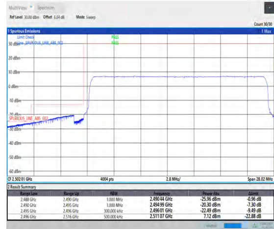
1-N41--30-20-L-6-CP-QPSK-Outer_Full-51@0-Ant t2-PASS-see graph
