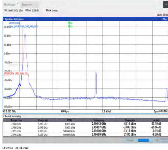
1-N41--30-60-L-4-CP-QPSK-Edge_1RB_Left-1@0-Ant 1-PASS-see graph
