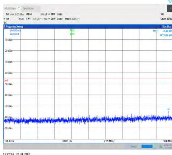
1-N41--30-100-M-1-DFT-QPSK-Edge_1RB_Left-1@ 0-0.15-30-Ant1--76.40--45-PASS
