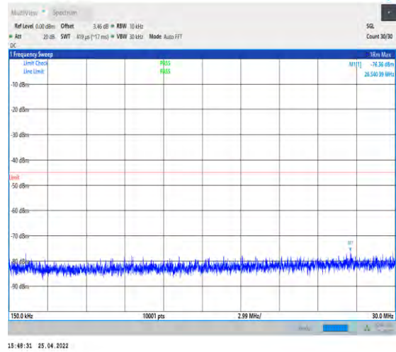
1-N41--30-100-H-1-DFT-QPSK-Edge_1RB_Left-1@ -0.15-30-Ant1--76.36--45-PASS
