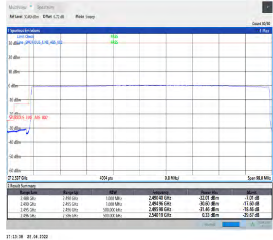
1-N41--30-90-L-6-CP-QPSK-Outer_Full-245@0-A nt1-PASS-see graph
