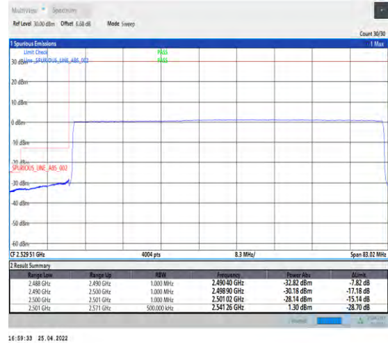
1-N41--30-70-L-6-CP-QPSK-Outer_Full-189@0-A nt1-PASS-see graph
