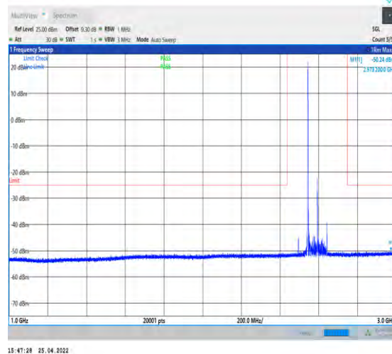
1-N41--30-100-M-1-DFT-QPSK-Edge_1RB_Left-1@ 0-1000-3000-Ant1--50.24--25-PASS
