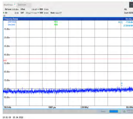
1-N41--30-100-M-1-DFT-QPSK-Edge_1RB_Left-1@ 0-0.15-30-Ant2--77.09--45-PASS
