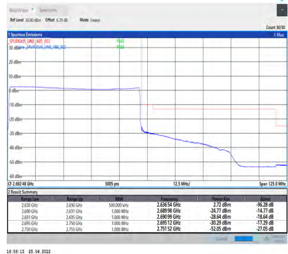
1-N41--30-60-H-6-CP-QPSK-Outer_Full-162@0-A nt1-PASS-see graph
