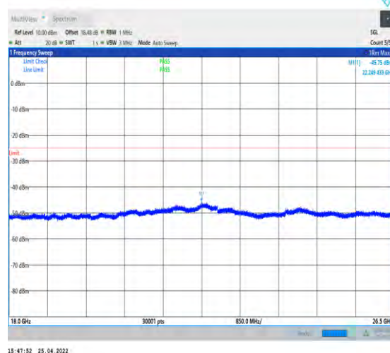
1-N41--30-100-M-1-DFT-QPSK-Edge_1RB_Left-1@ 0-18000-26500-Ant1--45.75--25-PASS
