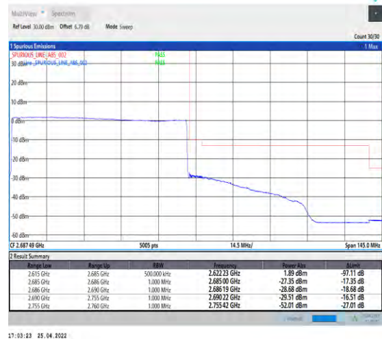
1-N41--30-70-H-6-CP-QPSK-Outer_Full-189@0-A nt1-PASS-see graph
