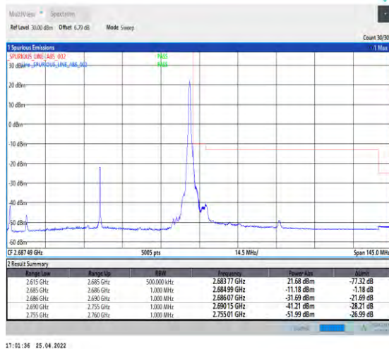
1-N41--30-70-H-5-CP-QPSK-Edge_1RB_Right-1@188-Ant nt1-PASS-see graph
