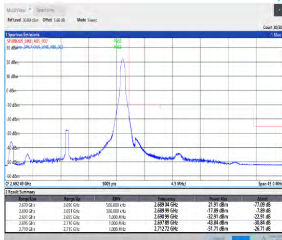
1-N41--30-20-H-5-CP-QPSK-Edge_1RB_Right-1@50-Ant Ant2-PASS-see graph
