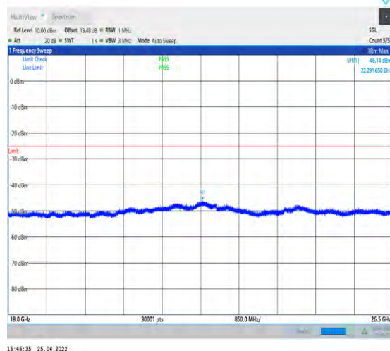
1-N41--30-100-L-1-DFT-QPSK-Edge_1RB_Left-1@ -18000-26500-Ant1--46.14--25-PASS
