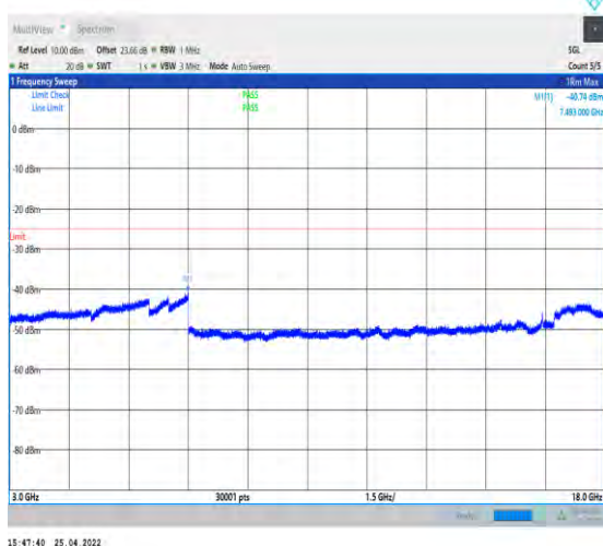
1-N41--30-100-M-1-DFT-QPSK-Edge_1RB_Left-1@ 0-3000-18000-Ant1--40.74--25-PASS
