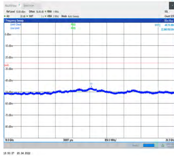
1-N41--30-100-L-1-DFT-QPSK-Edge_1RB_Left-1@ -18000-26500-Ant2--46.19--25-PASS
