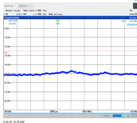
1-N41--30-100-M-1-DFT-QPSK-Edge_1RB_Left-1@ 0-18000-26500-Ant2--45.81--25-PASS
