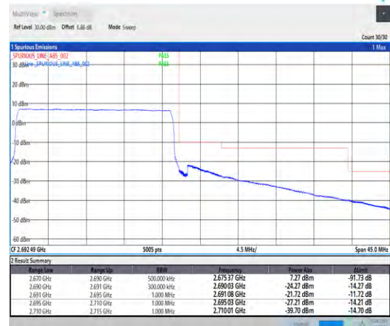
1-N41--30-20-H-6-CP-QPSK-Outer_Full-51@0-Ant t2-PASS-see graph
