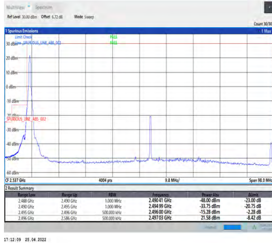
1-N41--30-90-L-4-CP-QPSK-Edge_1RB_Left-1@0-Ant 1-PASS-see graph
