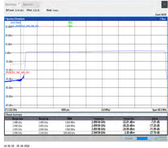
1-N41--30-60-L-6-CP-QPSK-Outer_Full-162@0-A nt1-PASS-see graph
