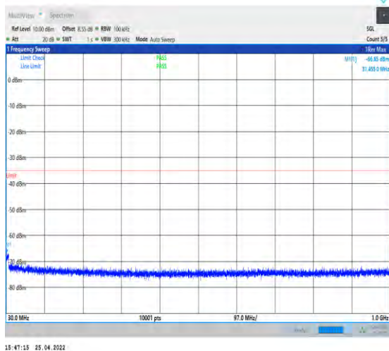
1-N41--30-100-M-1-DFT-QPSK-Edge_1RB_Left-1@ 0-30-1000-Ant1--66.85--35-PASS
