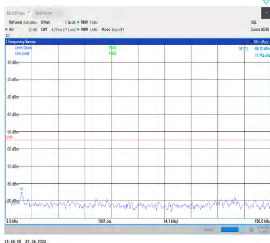
1-N41--30-100-M-1-DFT-QPSK-Edge_1RB_Left-1@ 0-0.009-0.15-Ant1--86.72--55-PASS
