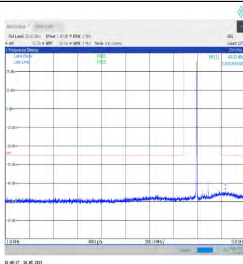
1-N41-30-100-H-1-DFT-PI2BPSK-Inner_1RB_Left-1 @1-1000-3000-Ant1--43.93--25-PASS
