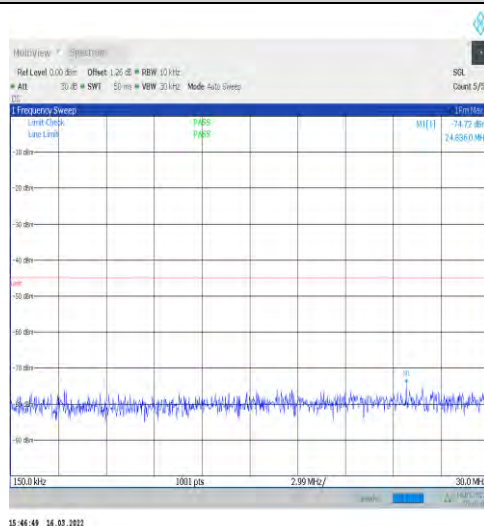
1-N41-30-100-M-1-DFT-PI2BPSK-Inner_1RB_Left-1 @1-0.15-30-Ant1--74.72--45-PASS
