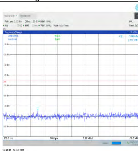
1-N41-30-100-H-1-DFT-PI2BPSK-Inner_1RB_Left-1 @1-0.15-30-Ant1--74.88--45-PASS
