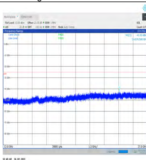
1-N41-30-100-L-1-DFT-PI2BPSK-Inner_1RB_Left-1 @1-12000-27000-Ant1--41.93--25-PASS
