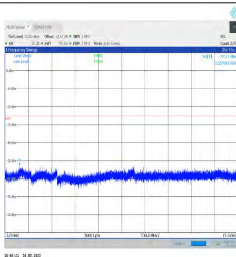
1-N41-30-100-L-1-DFT-PI2BPSK-Inner_1RB_Left-1 @1-3000-12000-Ant1--52.71--25-PASS
