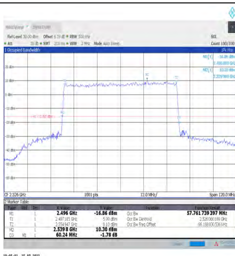
1-N41-30-60-L-9-CP-256QAM-Outer_Full-162@0-Ant t1-57.762-60.240-≤60-PASS
