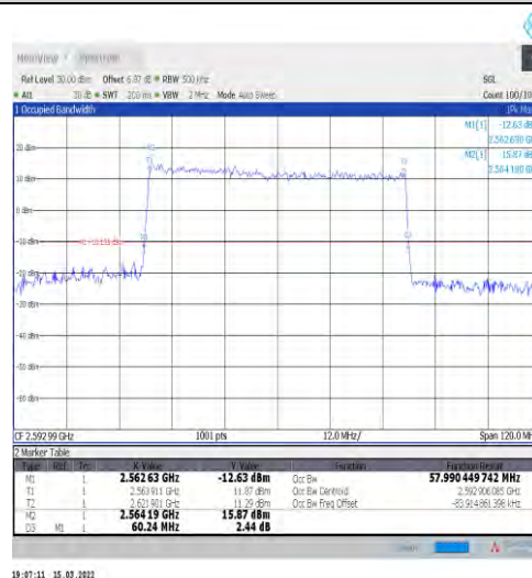
1-N41-30-60-M-3-DFT-16QAM-Outer_Full-162@0-Ant t1-57.99-60.240-≤60-PASS
