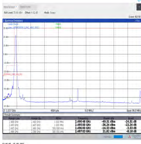
1-N41-30-90-L-1-DFT-PI2BPSK-Edge_1RB_Left-1@0-Ant1-PASS-see graph
