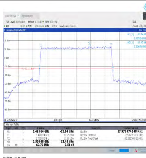
1-N41-30-60-L-4-DFT-64QAM-Outer_Full-162@0-Ant t1-57.978-60.720-≤60-PASS
