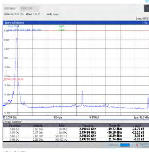
1-N41-30-90-L-4-CP-QPSK-Edge_1RB_Left-1@0-Ant1-PASS-see graph
