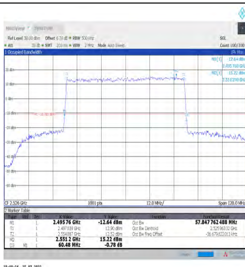
1-N41-30-60-L-1-DFT-QPSK-Outer_Full-162@0-Ant t1-57.848-60.480-≤60-PASS
