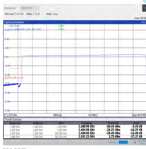
1-N41-30-60-L-6-CP-QPSK-Outer_Full-162@0-Ant1-PASS-see graph
