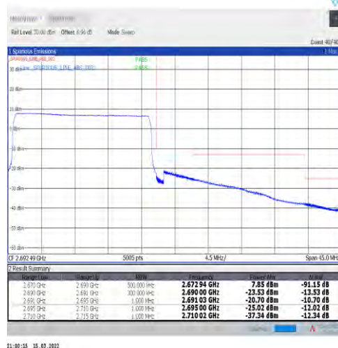
1-N41-30-20-H-6-CP-QPSK-Outer_Full-51@0-Ant1-PASS-see graph
