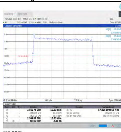
1-N41-30-60-M-1-DFT-QPSK-Outer_Full-162@0-Ant t1-57.825-60.360-≤60-PASS
