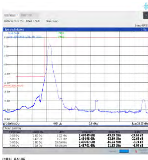
1-N41-30-20-L-4-CP-QPSK-Edge_1RB_Left-1@0-Ant1-PASS-see graph
