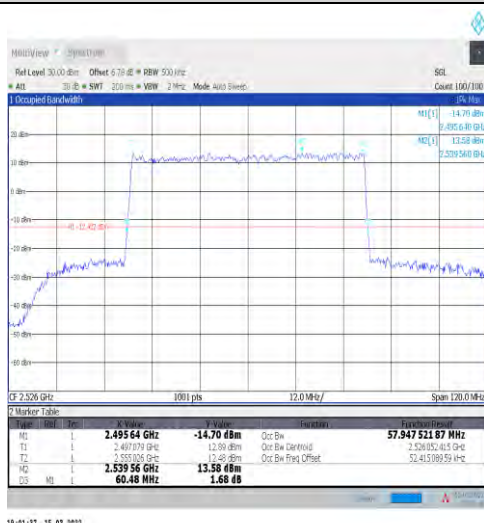
1-N41-30-60-L-3-DFT-16QAM-Outer_Full-162@0-Ant t1-57.948-60.480-≤60-PASS
