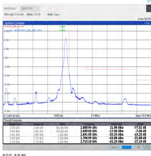
1-N41-30-20-H-5-CP-QPSK-Edge_1RB_Right-1@50-Ant1-PASS-see graph
