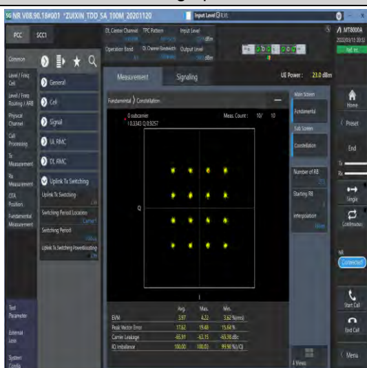
1-N41-30-100-M-7-CP-16QAM-Outer_Full-273@0-An t1-see graph-PASS
