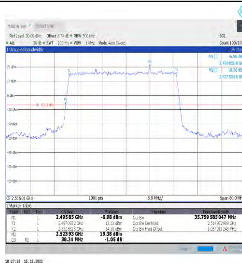
1-N41-30-40-L-2-DFT-PI2BPSK-Outer_Full-100@0-Ant1 1-35.76-38.240-≤40-PASS
