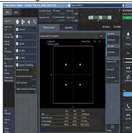
1-N41-30-100-M-6-CP-QPSK-Outer_Full-273@0-An t1-see graph-PASS
