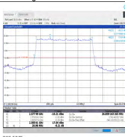
1-N41-30-30-M-2-DFT-PI2BPSK-Outer_Full-75@0-A nt1-26.859-28.980-≤30-PASS
