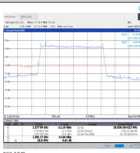
1-N41-30-30-M-4-DFT-64QAM-Outer_Full-75@0-Ant 1-26.836-28.800≤30-PASS
