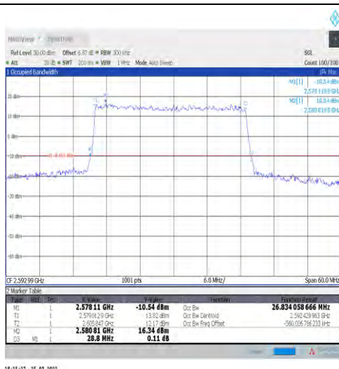
1-N41-30-30-M-1-DFT-QPSK-Outer_Full-75@0-Ant1 -26.834-28.800-≤30-PASS
