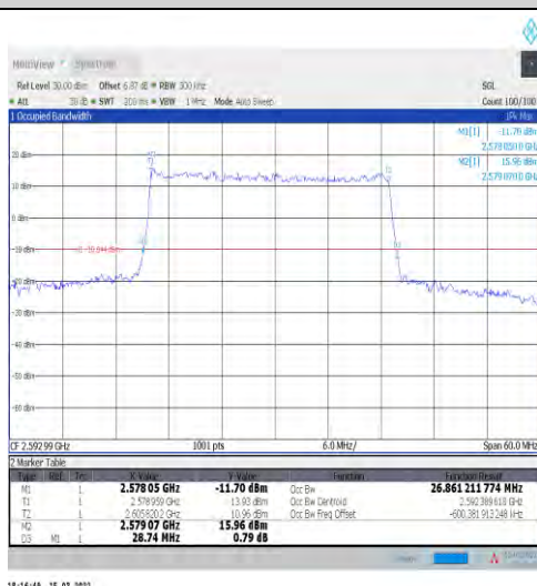
1-N41-30-30-M-3-DFT-16QAM-Outer_Full-75@0-Ant 1-26.861-28.740≤30-PASS
