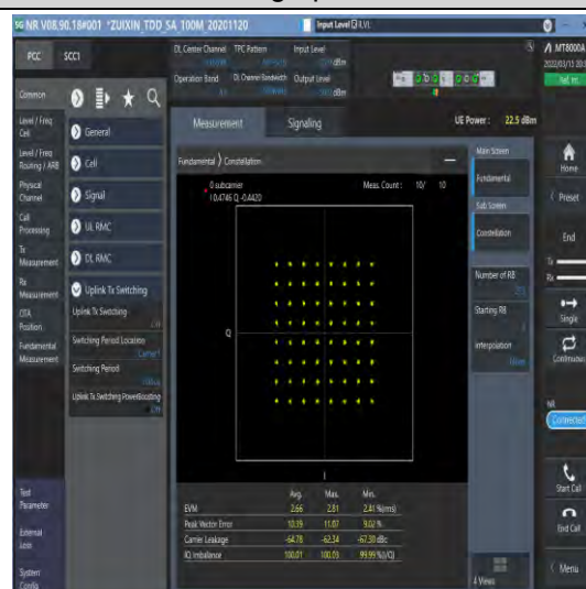
1-N41-30-100-M-8-CP-64QAM-Outer_Full-273@0- Ant1-see graph-PASS
