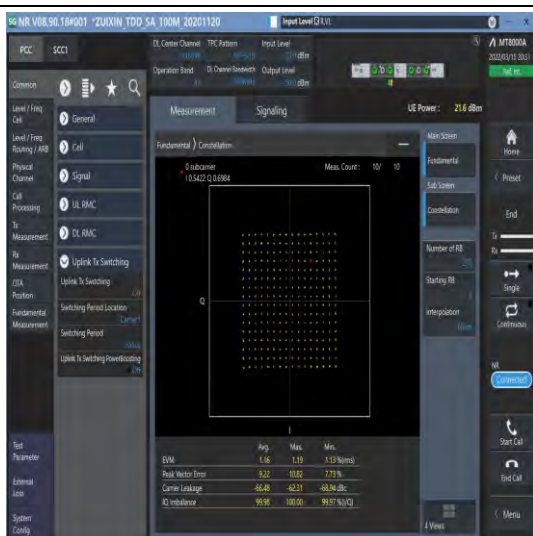
1-N41-30-100-M-5-DFT-256QAM-Outer_Full-270@0- Ant1-see graph-PASS
