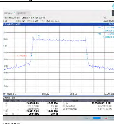
1-N41-30-30-H-9-CP-256QAM-Outer_Full-78@0-Ant1 1-27.836-29.640-≤30-PASS
