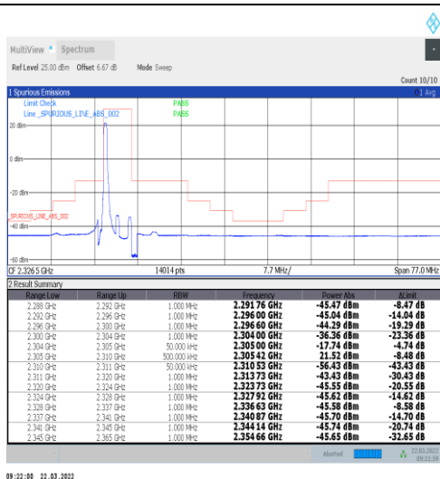
1-N30-15-5-L-1-DFT-PI2BPSK-Edge_1RB_Left-1@0-Ant1-PASS-see graph
