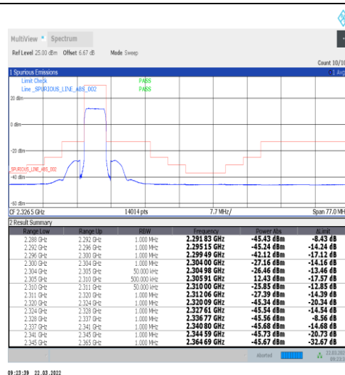
1-N30-15-5-L-3-DFT-PI2BPSK-Outer_Full-25@0-Ant1-PASS-see graph
