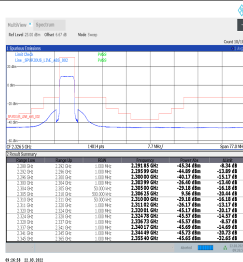
1-N30-15-5-L-6-CP-QPSK-Outer_Full-25@0-Ant1-PASS-see graph
