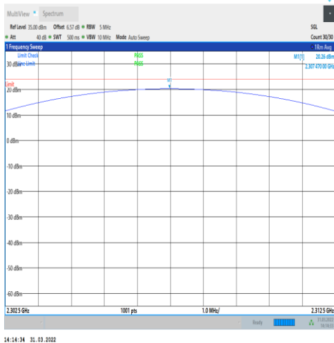
1-N30-PC3-15-5-L-3-DFT-PI2BPSK-Outer_Full-25 @0-2302.5-2312.5-Ant1-20.26-23.98-PASS
