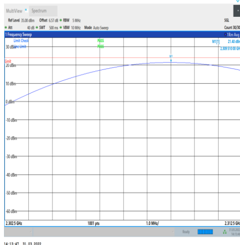
1-N30-PC3-15-5-L-2-DFT-PI2BPSK-Inner_1RB_Right t-1@23-2302.5-2312.5-Ant1-21.40-23.98-PASS
