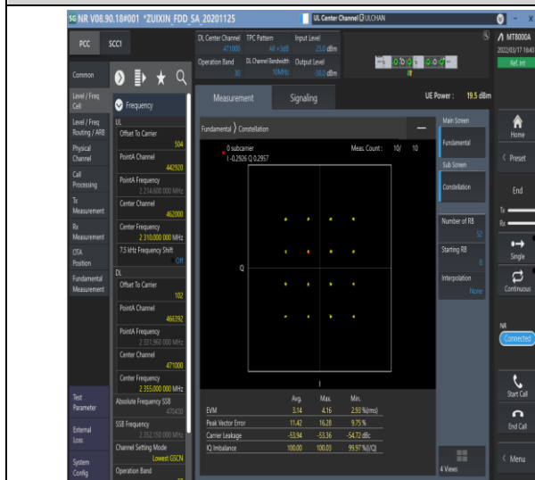
1-N30-15-10-M-7-CP-16QAM-Outer_Full-52@0-Ant1-see graph-PASS
