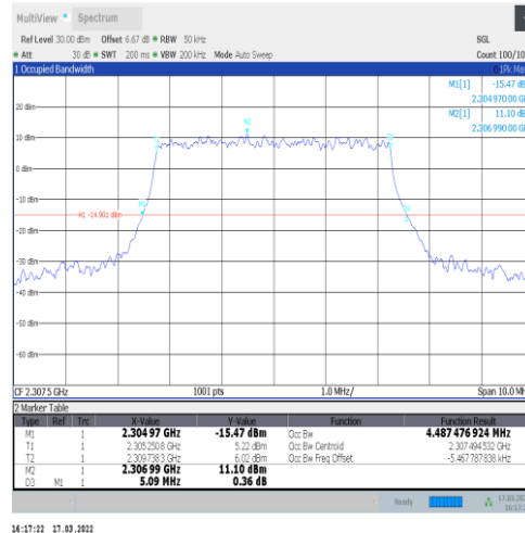
1-N30-15-5-L-4-DFT-64QAM-Outer_Full-25@0-Ant1 -4.487-5.090-≤5-PASS
