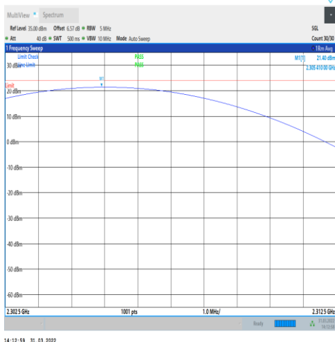
1-N30-PC3-15-5-L-1-DFT-PI2BPSK-Inner_1RB_Left -1@1-2302.5-2312.5-Ant1-21.40-23.98-PASS
