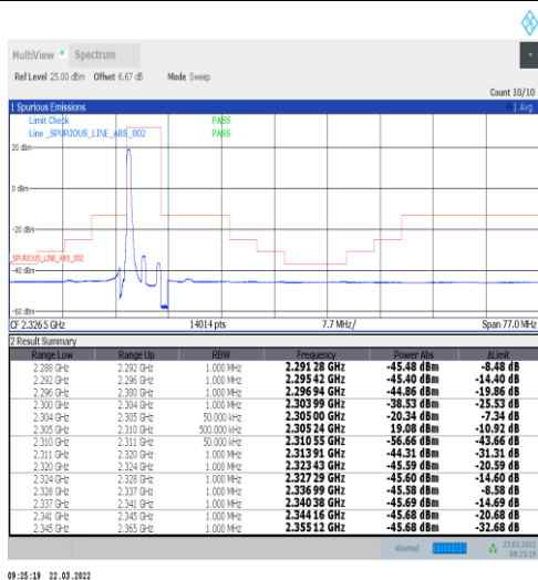
1-N30-15-5-L-4-CP-QPSK-Edge_1RB_Left-1@0-Ant1-PASS-see graph
