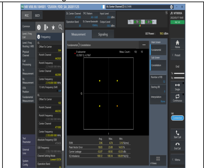
1-N30-15-10-M-6-CP-QPSK-Outer_Full-52@0-Ant1-see graph-PASS
