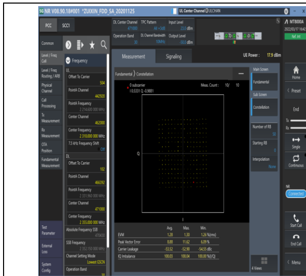
1-N30-15-10-M-5-DFT-256QAM-Outer_Full-50@0-Ant1-see graph-PASS
