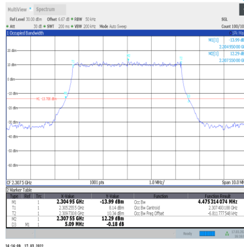
1-N30-15-5-L-2-DFT-PI2BPSK-Outer_Full-25@0-Ant 1-4.475-5.090-≤5-PASS
