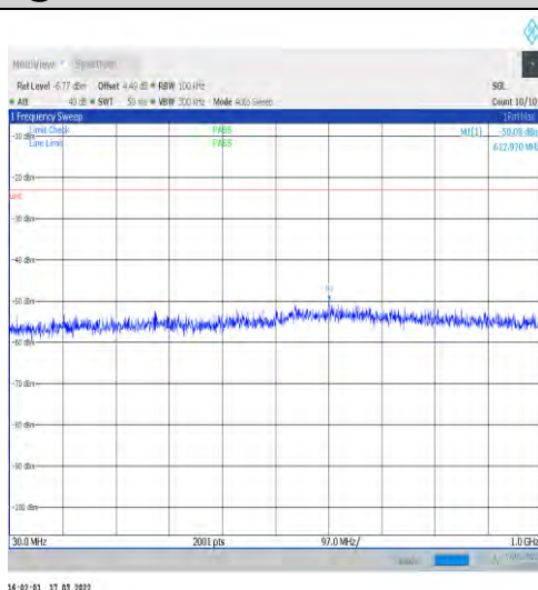
1-N25-15-40-H-1-DFT-PI2BPSK-Inner_1RB_Left-1 @1-30-1000-Ant1--50.08--23-PASS
