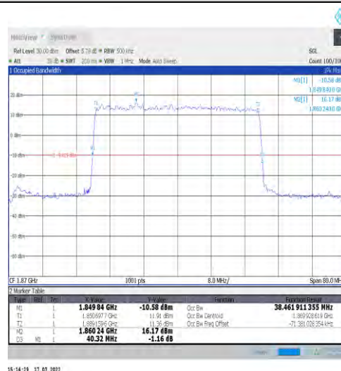
1-N25-15-40-L-2-DFT-PI2BPSK-Outer_Full-216@0-A Ant1-38.462-40.320-≤40-PASS
