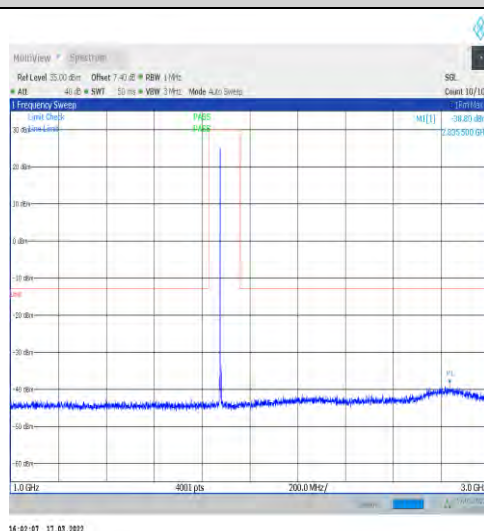
1-N25-15-40-H-1-DFT-PI2BPSK-Inner_1RB_Left-1@ 1-1000-3000-Ant1--38.80--13-PASS
