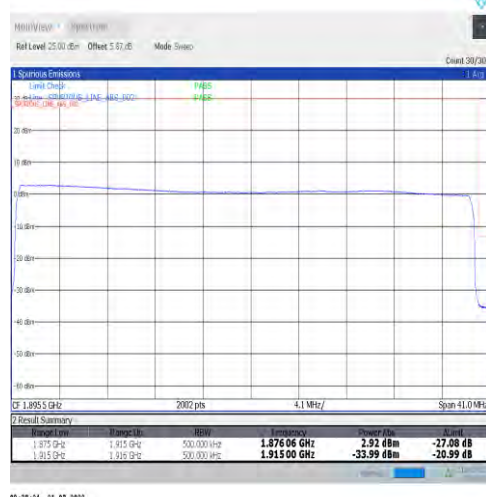
1-N25-15-40-H-6-CP-QPSK-Outer_Full-216@0-Ant1-seegraph-PASS-see graph
