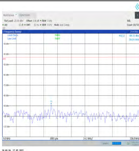
1-N25-15-40-M-1-DFT-PI2BPSK-Inner_1RB_Left-1@ 1-0.009-0.15-Ant1--88.72--43-PASS
