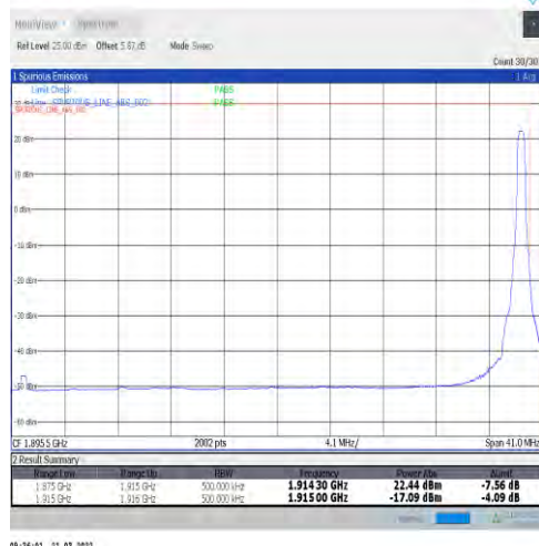
1-N25-15-40-H-2-DFT-PI2BPSK-Edge_1RB_Right-1@215-Ant1-seegraph-PASS-see graph
