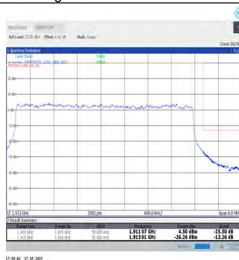
1-N25-15-5-H-3-DFT-PI2BPSK-Outer_Full-25@0- Ant1-seegraph-PASS-see graph
