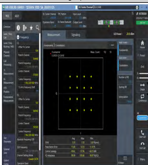
1-N25-15-40-M-7-CP-16QAM-Outer_Full-216@0-Ant 1-see graph-PASS
