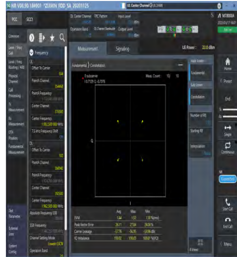
1-N25-15-40-M-2-DFT-QPSK-Outer_Full-216@0-An t1-see graph-PASS
