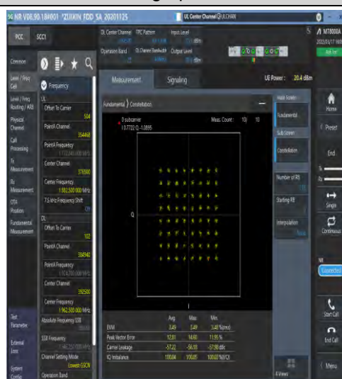
1-N25-15-40-M-8-CP-64QAM-Outer_Full-216@0-A nt1-see graph-PASS
