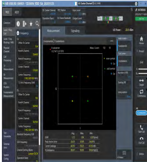
1-N25-15-40-M-1-DFT-PI2BPSK-Outer_Full-216@0- Ant1-see graph-PASS
