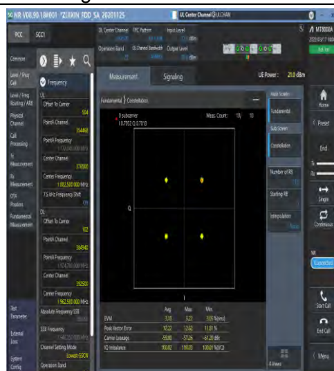
1-N25-15-40-M-6-CP-QPSK-Outer_Full-216@0-Ant 1-see graph-PASS
