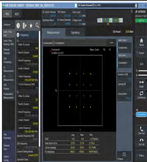
1-N25-15-40-M-3-DFT-16QAM-Outer_Full-216@0-An t1-see graph-PASS
