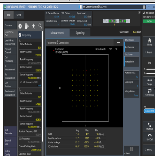
1-N14-15-10-M-8-CP-64QAM-Outer_Full-52@0-Ant1-see graph-PASS
