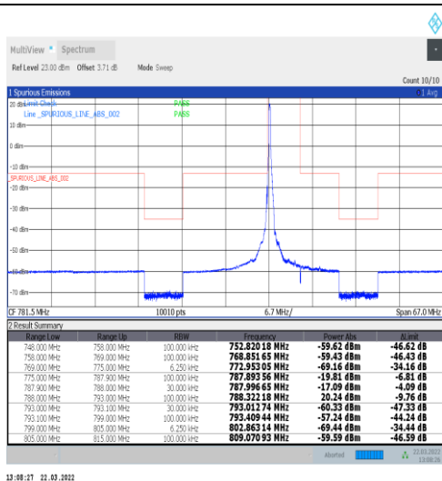
1-N14-15-5-L-1-DFT-PI2BPSK-Edge_1RB_Left-1@0-Ant1-PASS-see graph
