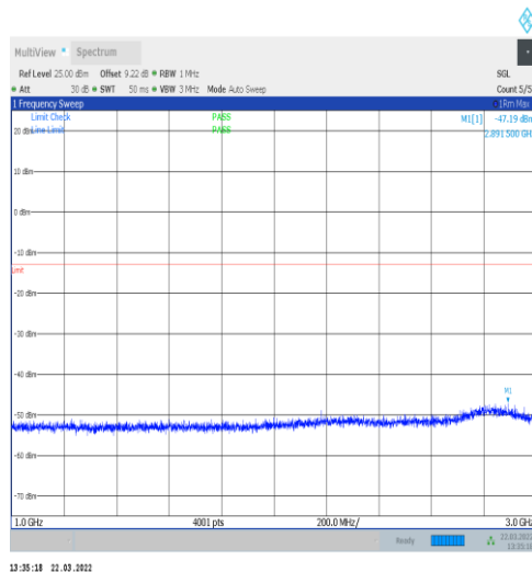
1-N14-15-10-M-1-DFT-PI2BPSK-Inner_1RB_Left-1 @1-1000-3000-Ant1--47.19--13-PASS
