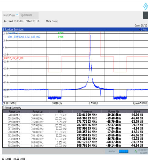
1-N14-15-5-L-4-CP-QPSK-Edge_1RB_Left-1@0-Ant1-PASS-see graph
