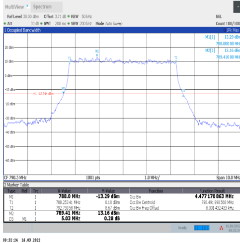
1-N14-15-5-L-1-DFT-QPSK-Outer_Full-25@0-Ant1-4 .477-5.030-≤5-PASS
