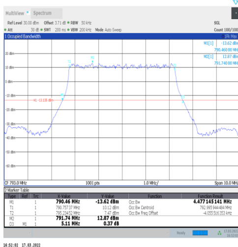
1-N14-15-5-M-2-DFT-PI2BPSK-Outer_Full-25@0-An t1-4.477-5.110-≤5-PASS
