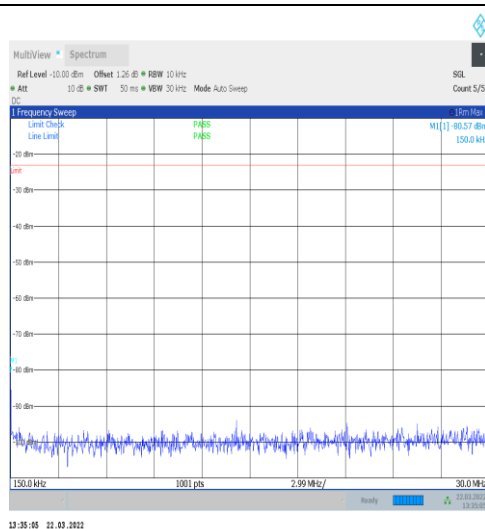
1-N14-15-10-M-1-DFT-PI2BPSK-Inner_1RB_Left-1 @1-0.15-30-Ant1--80.57--23-PASS
