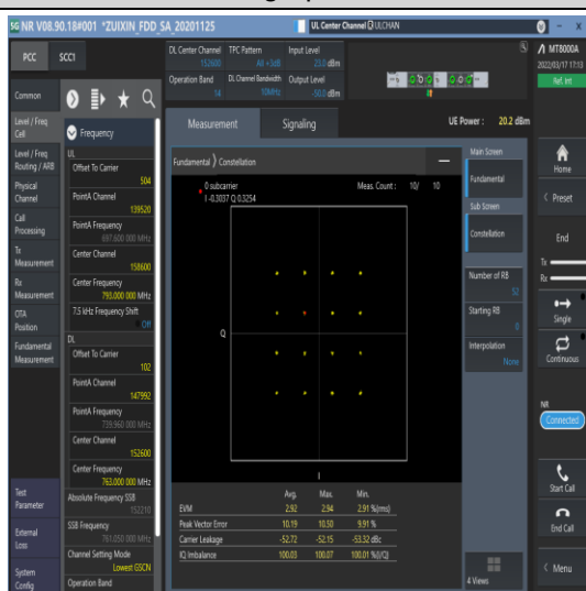
1-N14-15-10-M-7-CP-16QAM-Outer_Full-52@0-Ant1-see graph-PASS
