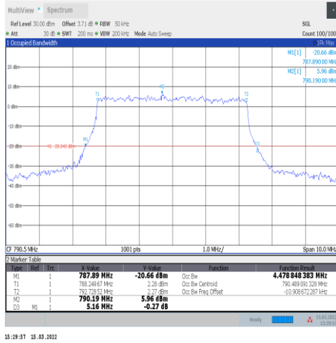
1-N14-15-5-L-9-CP-256QAM-Outer_Full-25@0-Ant1-4.479-5.160-≤5-PASS
