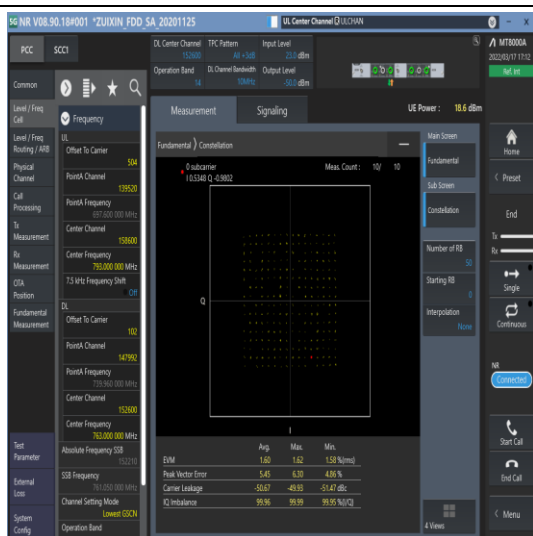
1-N14-15-10-M-5-DFT-256QAM-Outer_Full-50@0-Ant1-see graph-PASS
