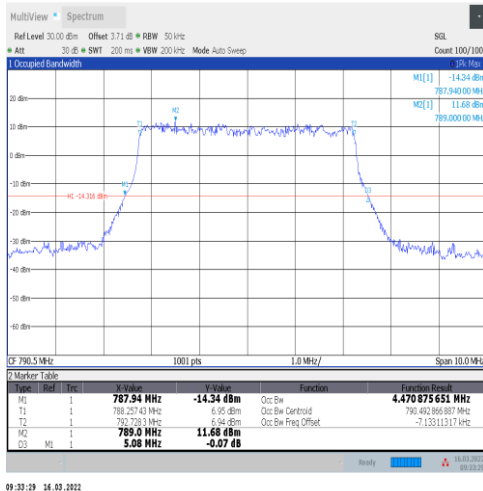
1-N14-15-5-L-3-DFT-16QAM-Outer_Full-25@0-Ant1-4 4.471-5.080-≤5-PASS
