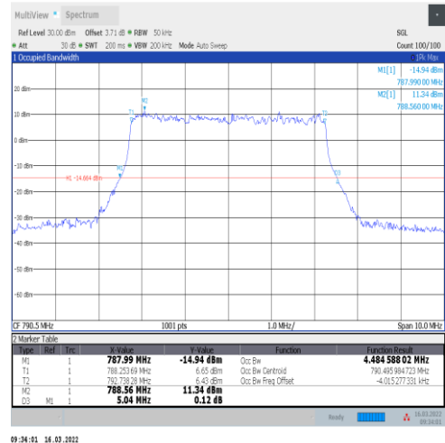
1-N14-15-5-L-4-DFT-64QAM-Outer_Full-25@0-Ant1-4 -4.485-5.040-≤5-PASS
