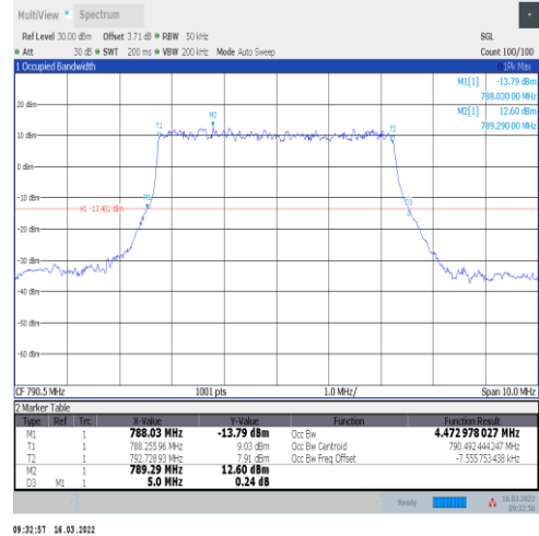
1-N14-15-5-L-2-DFT-PI2BPSK-Outer_Full-25@0-Ant1-4 1-4.473-5.000-≤5-PASS
