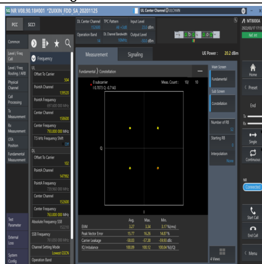
1-N14-15-10-M-6-CP-QPSK-Outer_Full-52@0-Ant1-see graph-PASS
