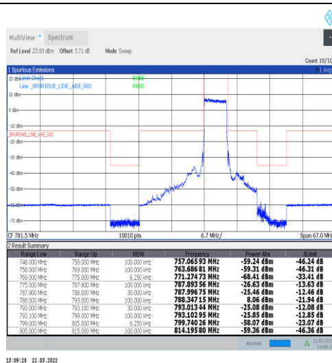
1-N14-15-5-L-3-DFT-PI2BPSK-Outer_Full-25@0-Ant1-PASS-see graph
