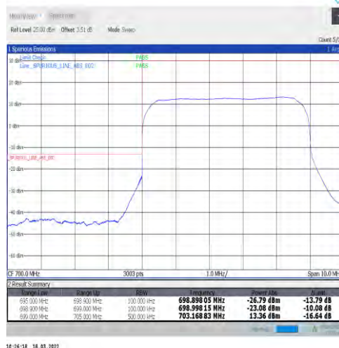
1-N12-15-5-L-3-DFT-PI2BPSK-Outer_Full-25@0-Ant1-PASS-see graph
