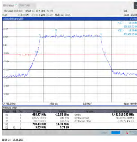
1-N12-15-5-L-1-DFT-QPSK-Outer_Full-25@0-Ant1-4 -4.481-5.030-≤5-PASS
