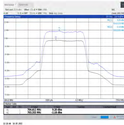
1-N12-15-15-L-2-CP-256QAM-Outer_Full-79@0-Ant 1-11.38-100%-0.00-11.38-PASS-≤13
