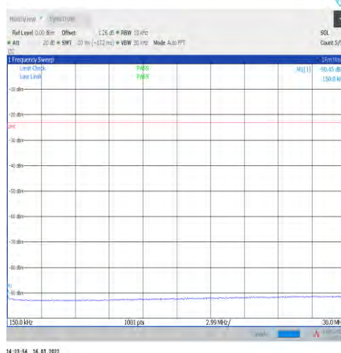
1-N5-15-20-H-1-DFT-PI2BPSK-Inner_1RB_Left-1@ 1-0.15-30-Ant1--90.45--23-PASS
