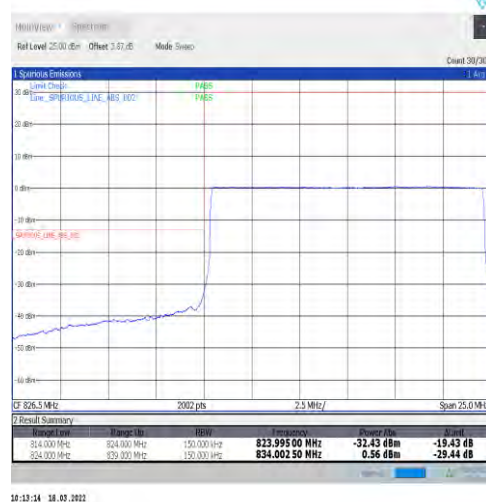
1-N5-15-15-L-6-CP-QPSK-Outer_Full-79@0-Ant1-seegraph-PASS-see graph
