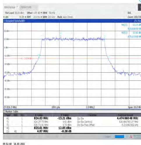
1-N5-15-5-L-2-DFT-PI2BPSK-Outer_Full-25@0-Ant1 -4.474-4.970-≤5-PASS
