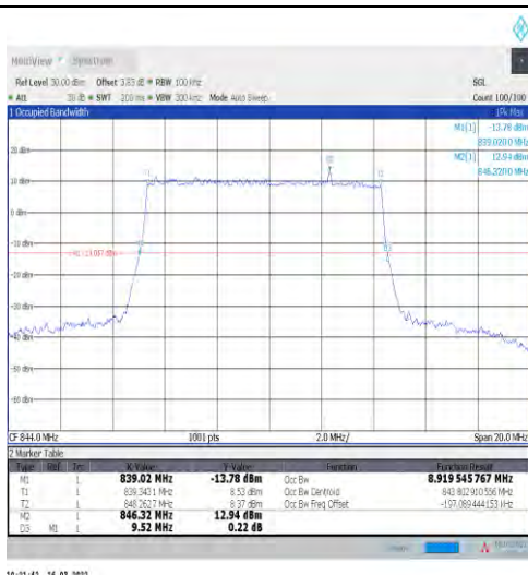
1-N5-15-10-H-4-DFT-64QAM-Outer_Full-50@0-Ant1 -8.92-9.520-≤10-PASS
