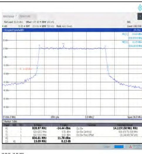
1-N5-15-15-M-6-CP-QPSK-Outer_Full-79@0-Ant1-1 4.119-15.090-≤15-PASS
