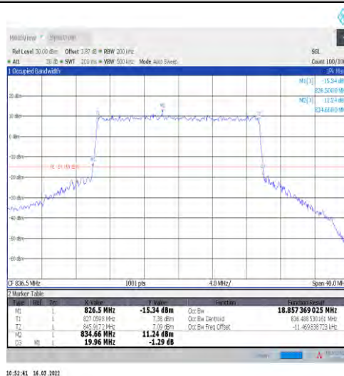
1-N5-15-20-M-6-CP-QPSK-Outer_Full-106@0-Ant 1-18.857-19.960-≤20-PASS
