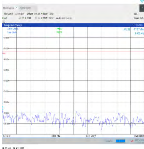
1-N5-15-20-H-1-DFT-PI2BPSK-Inner_1RB_Left-1@ 1-0.009-0.15-Ant1--87.97--33-PASS
