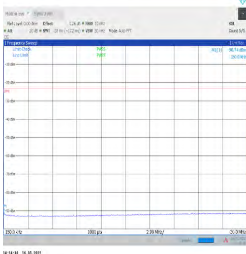
1-N5-15-20-M-1-DFT-PI2BPSK-Inner_1RB_Left-1@1 1-0.15-30-Ant1--90.74--23-PASS
