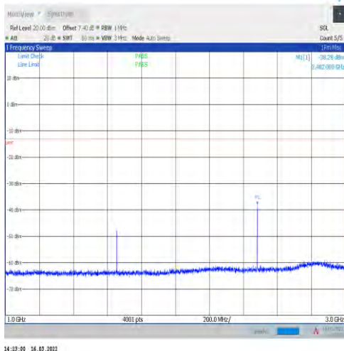
1-N5-15-20-M-1-DFT-PI2BPSK-Inner_1RB_Left-1@ 1-1000-3000-Ant1--38.28--13-PASS
