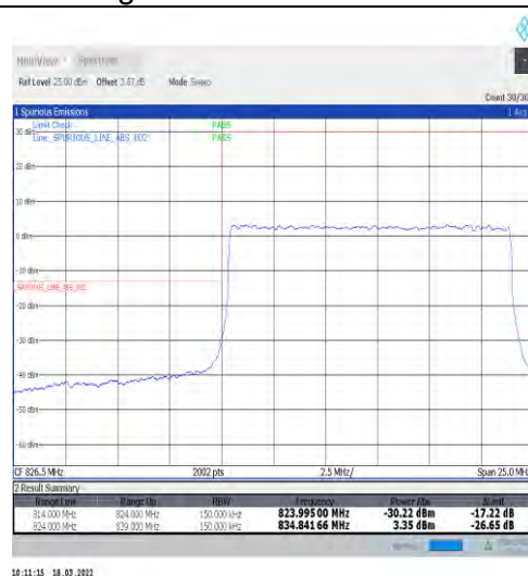
1-N5-15-15-L-3-DFT-PI2BPSK-Outer_Full-75@0-Ant1-seegraph-PASS-see graph
