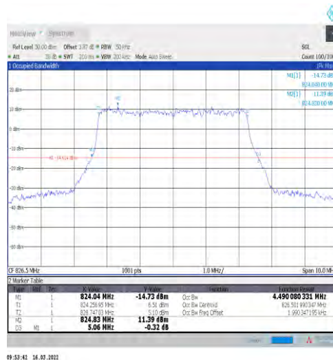
1-N5-15-5-L-4-DFT-64QAM-Outer_Full-25@0-Ant1-4 .49-5.060-≤5-PASS
