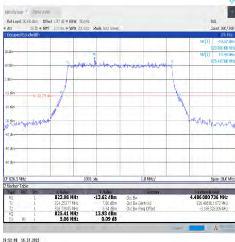
1-N5-15-5-L-1-DFT-QPSK-Outer_Full-25@0-Ant1-4. 486-5.060-≤5-PASS
