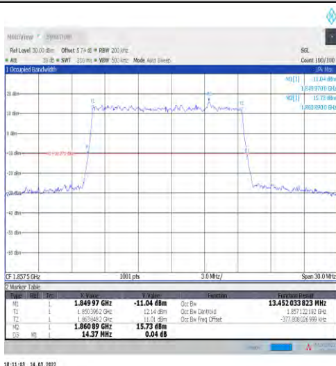
1-N2-15-15-L-1-DFT-QPSK-Outer_Full-75@0-Ant1-1-3.452-14.370-≤15-PASS
