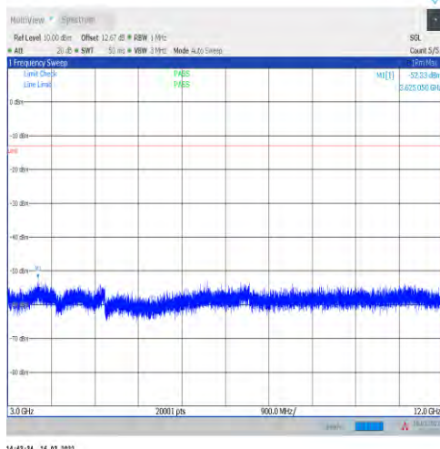
1-N2-15-20-H-1-DFT-PI2BPSK-Inner_1RB_Left-1@ 1-3000-12000-Ant1--52.33--13-PASS
