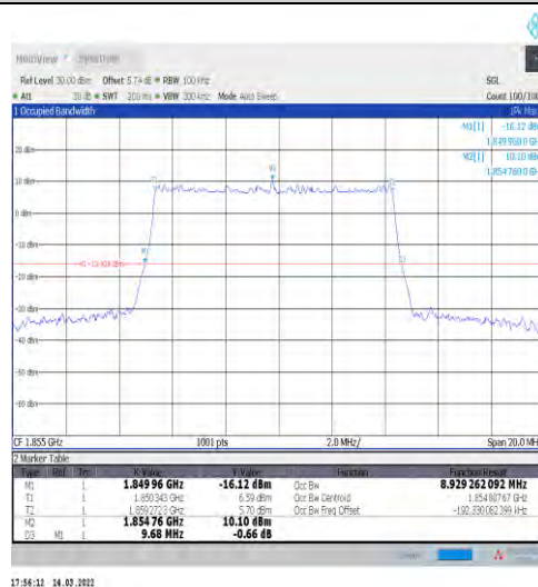
1-N2-15-10-L-5-DFT-256QAM-Outer_Full-50@0-Ant 1-8.929-9.680-≤10-PASS
