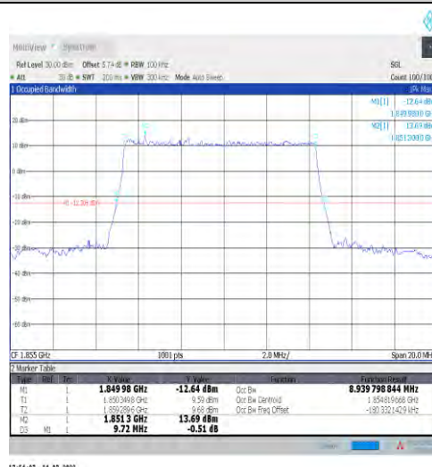
1-N2-15-10-L-1-DFT-QPSK-Outer_Full-50@0-Ant1-8 .94-9.720-≤10-PASS
