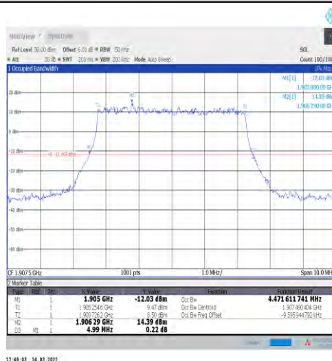
1-N2-15-5-H-2-DFT-PI2BPSK-Outer_Full-25@0-Ant1 -4.472-4.990≤5-PASS
