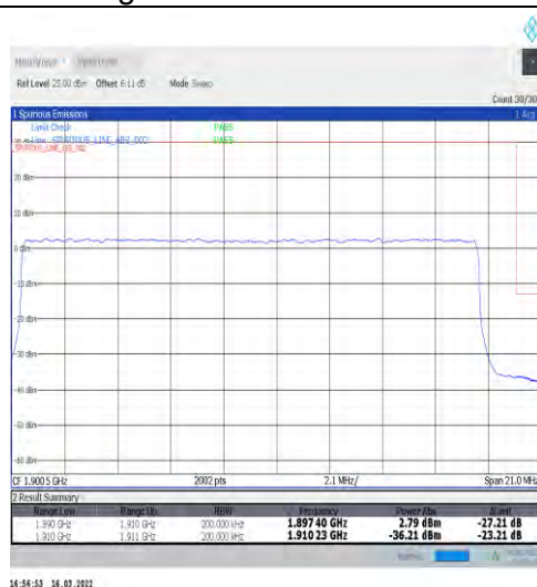
1-N2-15-20-H-3-DFT-PI2BPSK-Outer_Full-100@0-Ant1-seegraph-PASS-see graph
