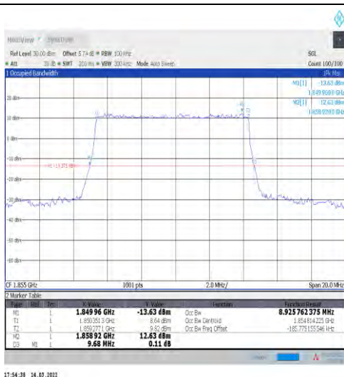
1-N2-15-10-L-2-DFT-PI2BPSK-Outer_Full-50@0-Ant 1-8.926-9.680-≤10-PASS
