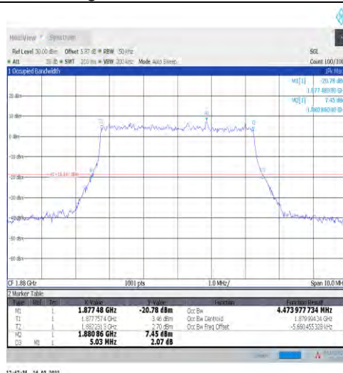
1-N2-15-5-M-9-CP-256QAM-Outer_Full-25@0-Ant1-4 4.474-5.030≤5-PASS
