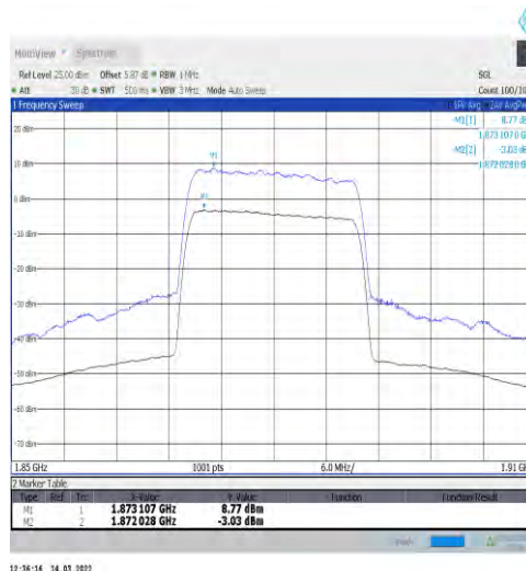
1-N2-15-20-M-2-CP-256QAM-Outer_Full-106@0-Ant t1-11.80-100%-0.00-11.80-PASS-≤13
