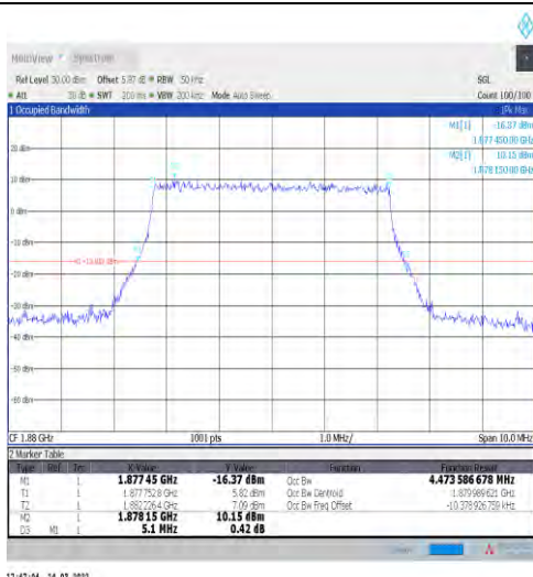
1-N2-15-5-M-8-CP-64QAM-Outer_Full-25@0-Ant1-4 4.474-5.100≤5-PASS
