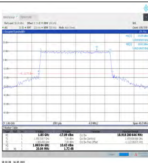
1-N2-15-20-L-8-CP-64QAM-Outer_Full-106@0-Ant1 -18.918-20.040-≤20-PASS
