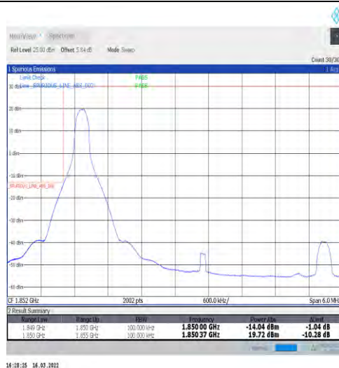
1-N2-15-5-L-1-DFT-PI2BPSK-Edge_1RB_Left-1@0-Ant1-seegraph-PASS-see graph
