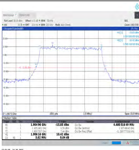
1-N2-15-5-H-7-CP-16QAM-Outer_Full-25@0-Ant1-4. 481-5.020-≤5-PASS
