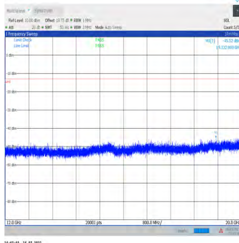
1-N2-15-20-H-1-DFT-PI2BPSK-Inner_1RB_Left-1@ 1-12000-20000-Ant1--45.52--13-PASS
