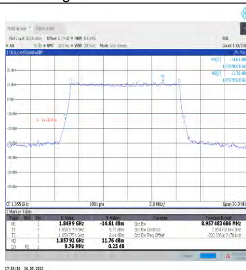
1-N2-15-10-L-3-DFT-16QAM-Outer_Full-50@0-Ant1- 8.957-9.760-≤10-PASS
