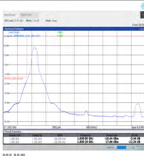
1-N2-15-5-L-4-CP-QPSK-Edge_1RB_Left-1@0-Ant1-seegraph-PASS-see graph
