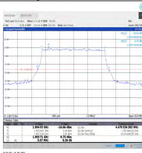
1-N2-15-5-H-8-CP-64QAM-Outer_Full-25@0-Ant1-4. 471-5.070-≤5-PASS
