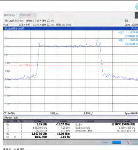
1-N2-15-20-L-3-DFT-16QAM-Outer_Full-100@0-Ant 1-17.879-18.920-≤20-PASS
