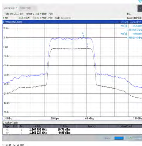
1-N2-15-20-L-1-DFT-256QAM-Outer_Full-100@0-Ant t1-11.71-100%-0.00-11.71-PASS-≤13
