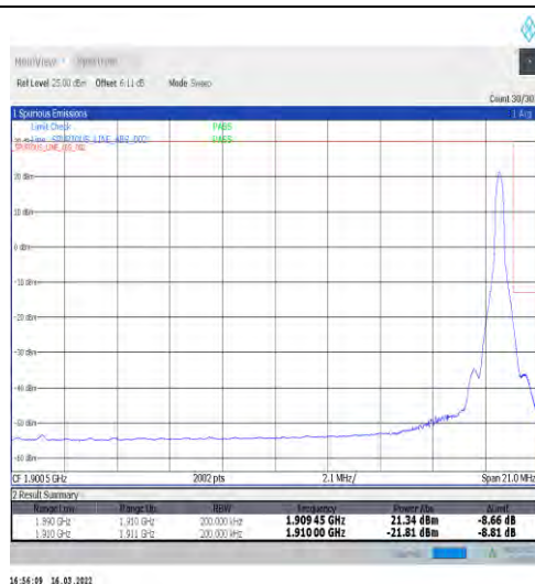
1-N2-15-20-H-2-DFT-PI2BPSK-Edge_1RB_Right-1@105-Ant1-seegraph-PASS-see graph
