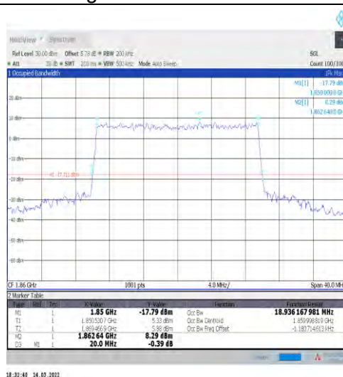
1-N2-15-20-L-9-CP-256QAM-Outer_Full-106@0-Ant1 1-18.936-20.000-≤20-PASS
