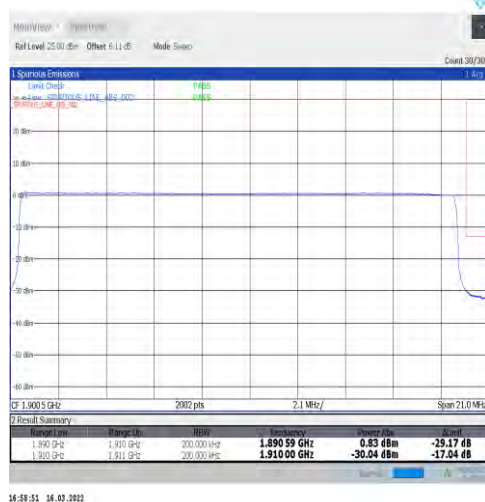
1-N2-15-20-H-6-CP-QPSK-Outer_Full-106@0-Ant1-seegraph-PASS-see graph
