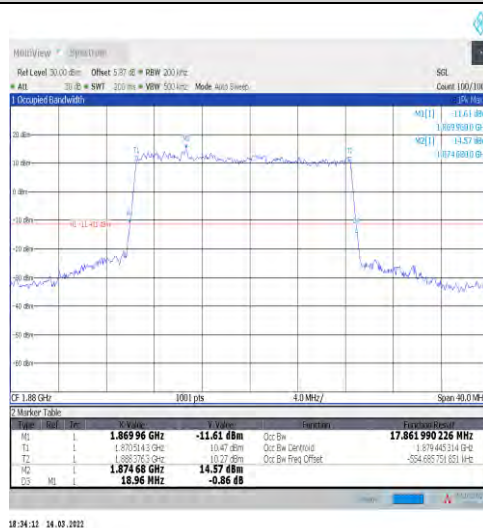
1-N2-15-20-M-2-DFT-PI2BPSK-Outer_Full-100@0-Ant1 -17.862-18.960-≤20-PASS
