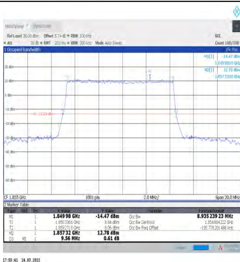
1-N2-15-10-L-4-DFT-64QAM-Outer_Full-50@0-Ant1 -8.935-9.560-≤10-PASS
