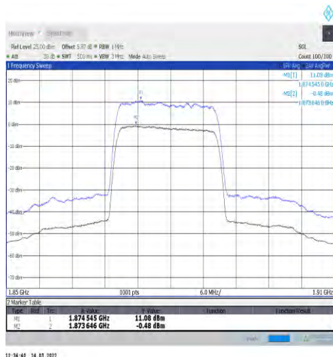
1-N2-15-20-M-1-DFT-256QAM-Outer_Full-100@0-A nt1-11.56-100%-0.00-11.56-PASS-≤13
