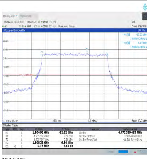
1-N2-15-5-H-9-CP-256QAM-Outer_Full-25@0-Ant1-4. 4.472-5.070-≤5-PASS
