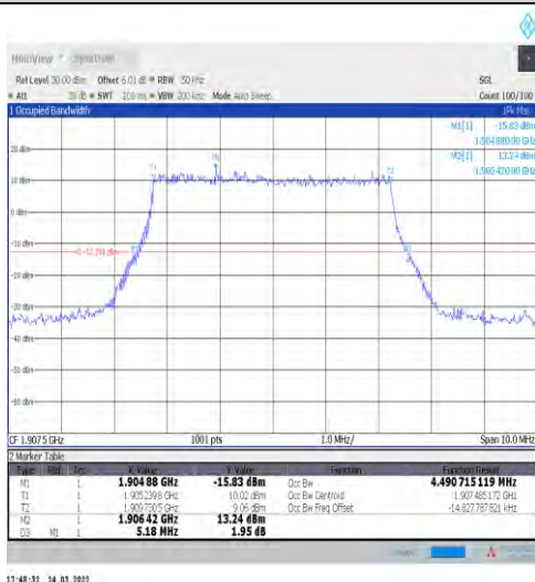
1-N2-15-5-H-1-DFT-QPSK-Outer_Full-25@0-Ant1-4. 491-5.180≤5-PASS
