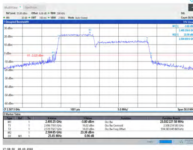
41-41-10MHz-15MHz-QPSK-QPSK-40549-40669-50RB#0-75RB#0
