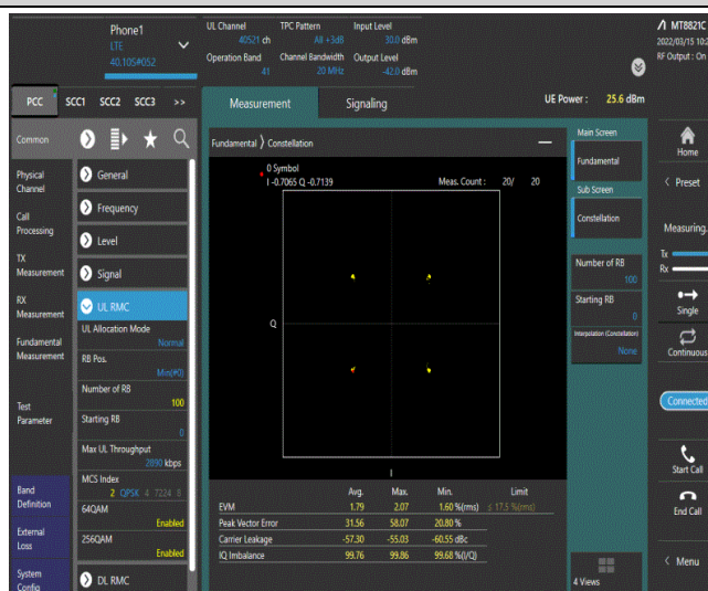
41-41-20MHz-20MHz-16QAM-QPSK-40521-40719
