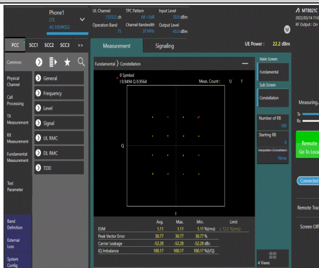
Band71-20MHz-16QAM-133322-100RB#0
