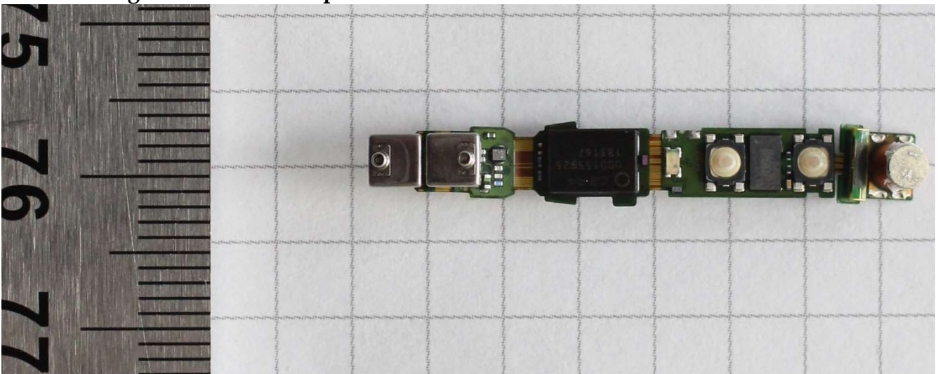
PCB showing button and microphone side
