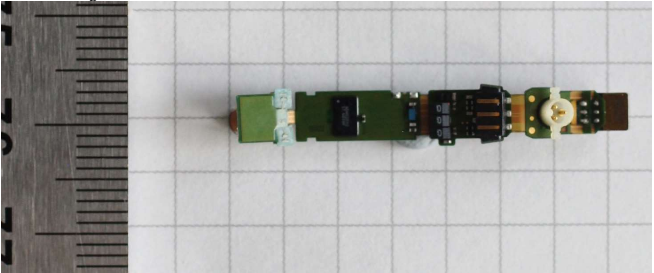
PCB showing the connector side
