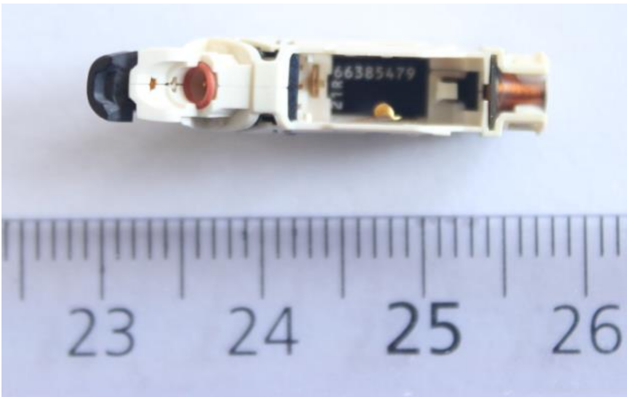
Bottom side with interface for speakers (left). Telecoil at right.
