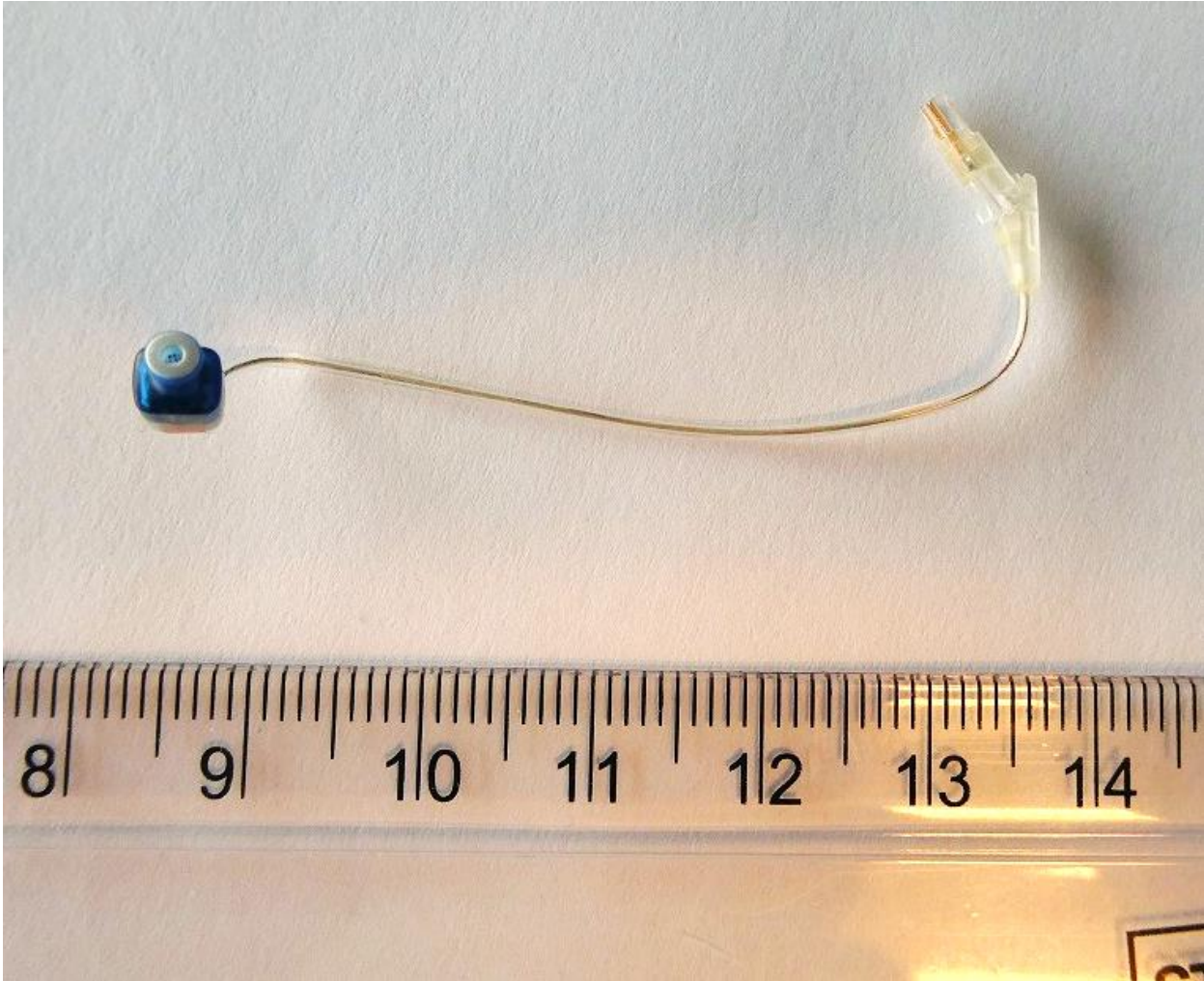
Speaker wire and Bluetooth (2.4 GHz) antenna with proprietary connector (L5)
