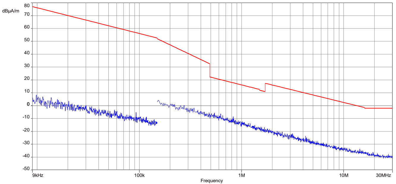
Plot 1: 9 kHz – 30 MHz; magnetic IC
