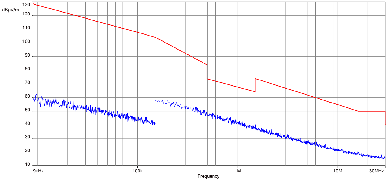
Plot 1: 9 kHz – 30 MHz; magnetic FCC
