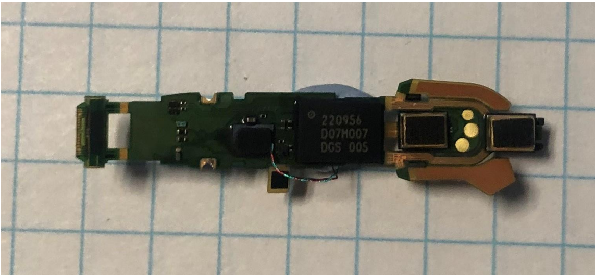
Bottom view PA_AU5_MBTE_M_R
