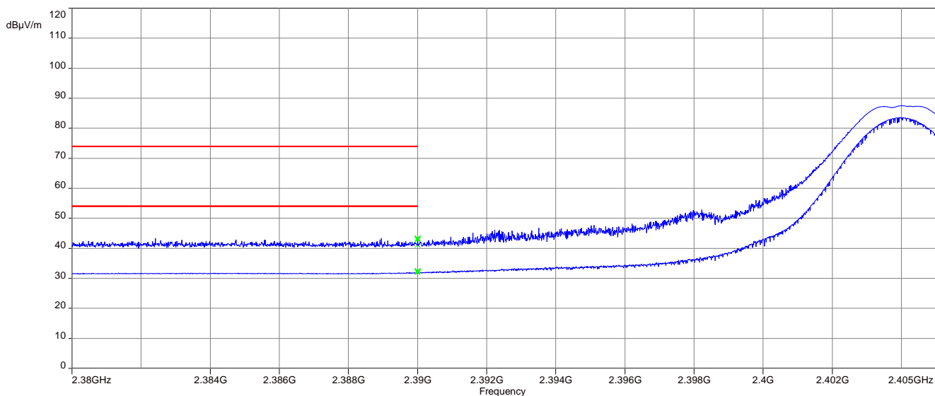
Plot 4: Lower restricted band, 2 Msp/s
