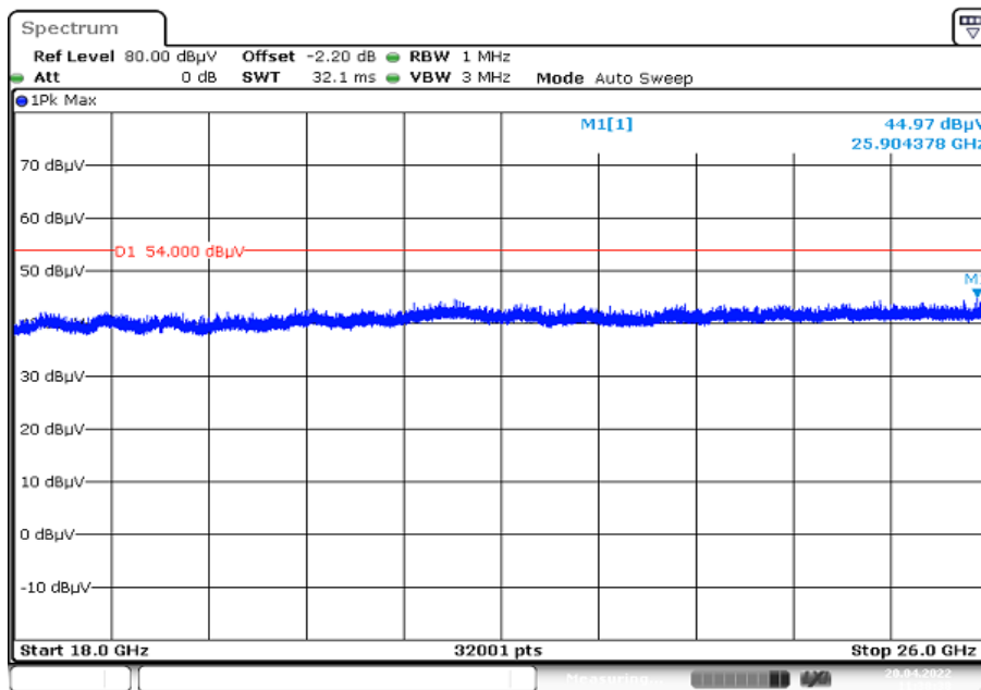
Plot 7: 18 GHz to 26 GHz, TX mode, vertical & horizontal polarization, valid for all channels of both modes
