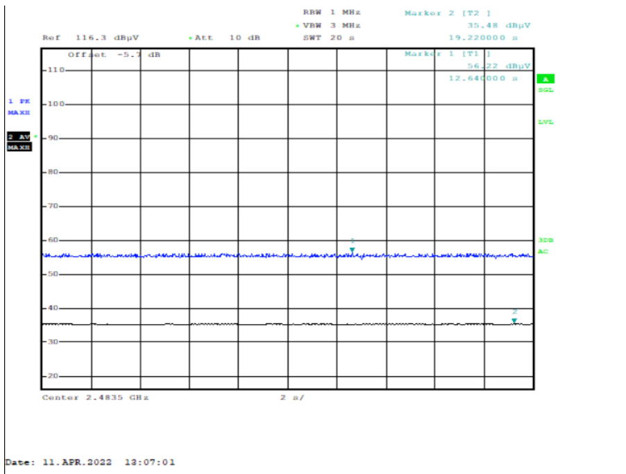
Plot 3: Upper restricted band, 1 Msp/s, detailed plot
