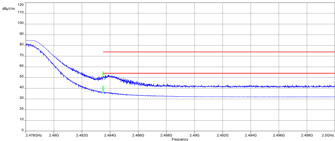
Plot 5: Upper restricted band, 2 Msps
