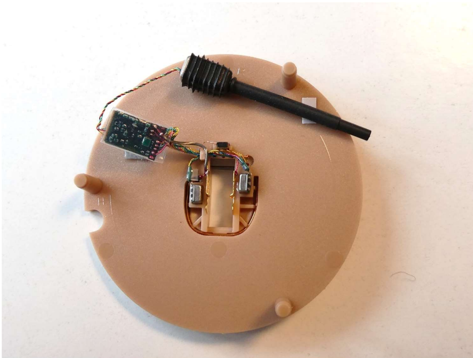
The AM_AU5_KIT312 hearing aid module stack up on faceplate (AU5 back side)
