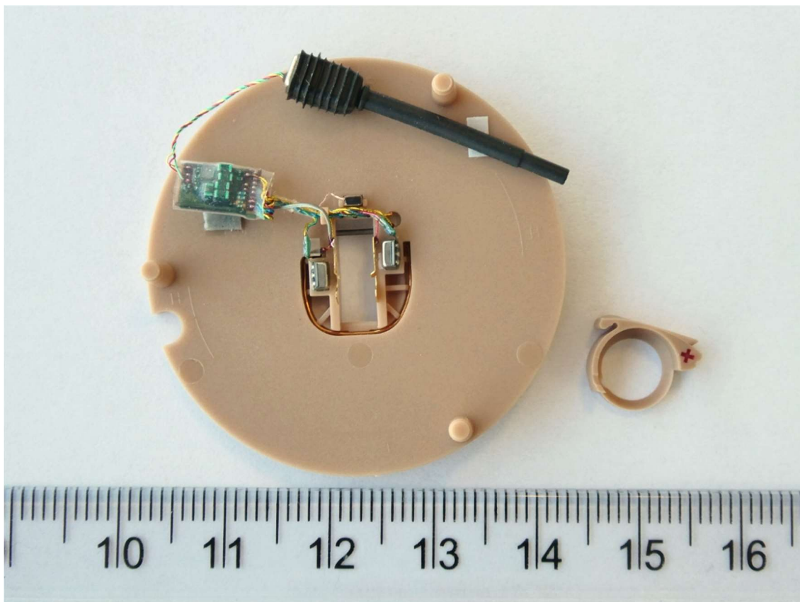
The AM_AU5_KIT312 hearing aid module stack up on faceplate, front-back
