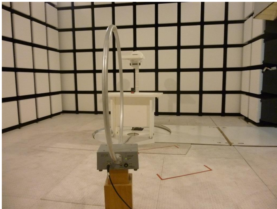
Photo 5: EUT at the anechoic chamber, loop antenna test setup
