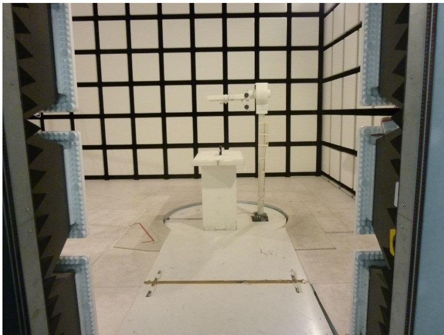
Photo 1: EUT at the anechoic chamber, loop antenna test setup
