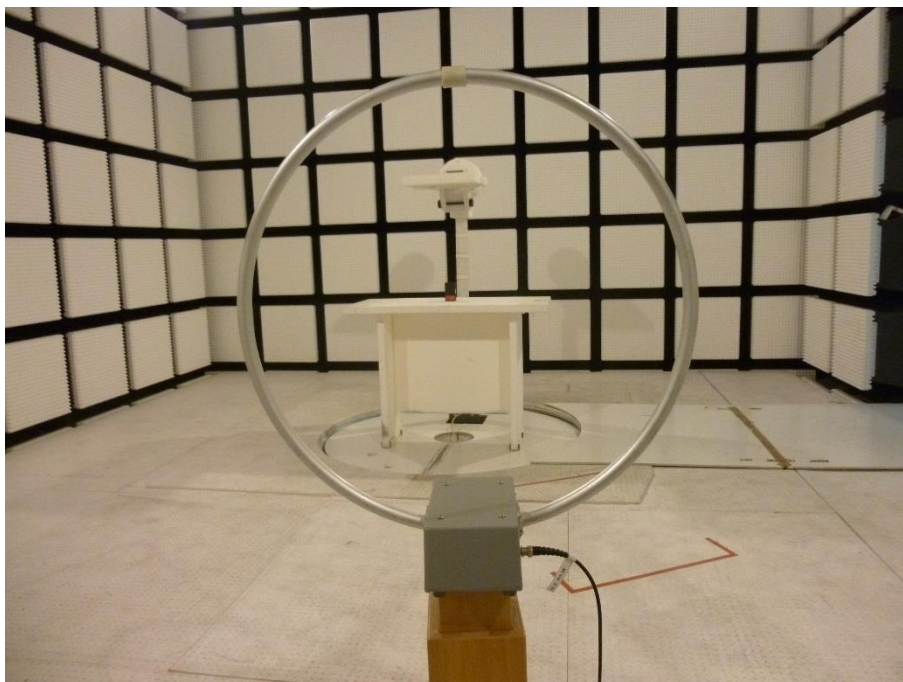
Photo 4: EUT at the anechoic chamber, loop antenna test setup
