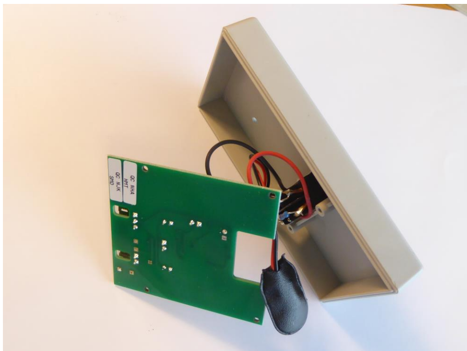
SBO Range Tester NL 4 PCB removed
