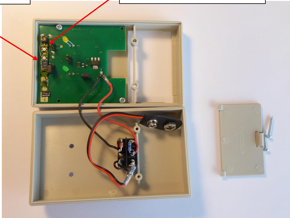
SBO Range Tester NL 4 open with ON/OFF button in the lid
