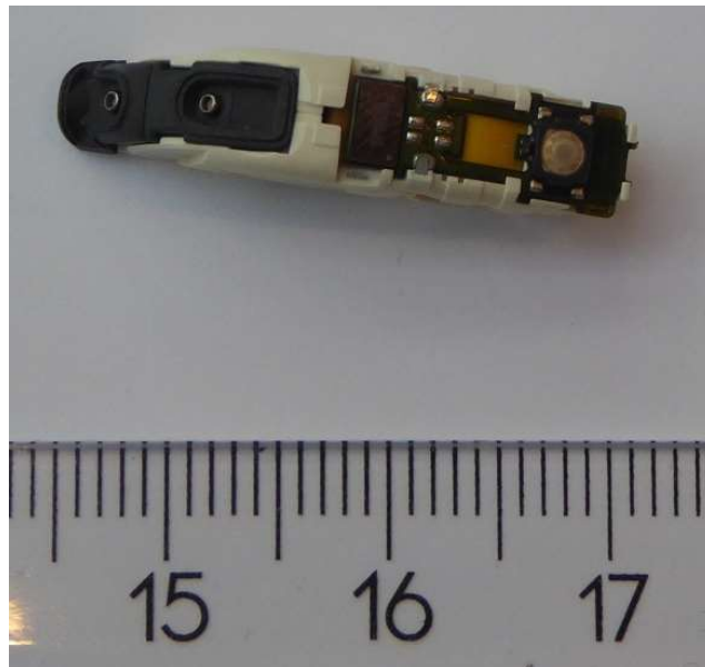
Radio module from the top side (button side)
