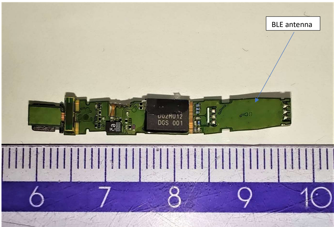
PCB showing the connector side
