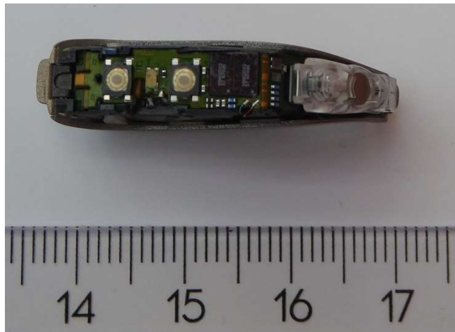
Radio module from the top side (button side)
