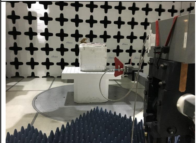
Radiated Spurious emission above 1G - Front View
