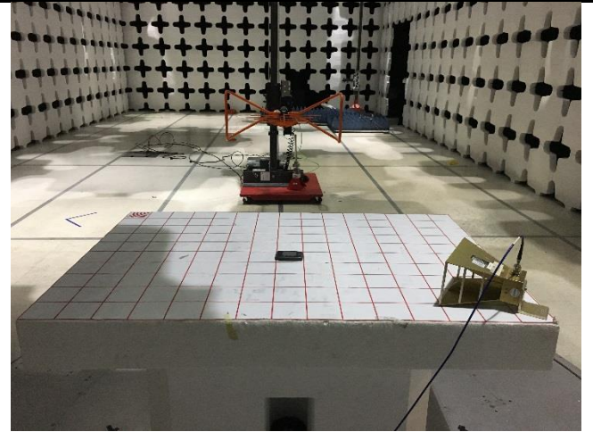
Radiated Spurious emission below 1G - Rear View
