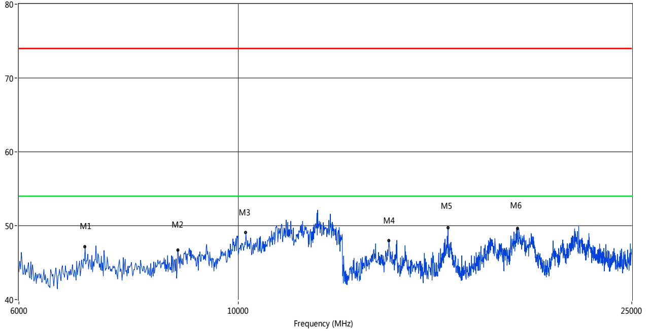
RE Test case_FCC 15C 6GHz-25GHz
