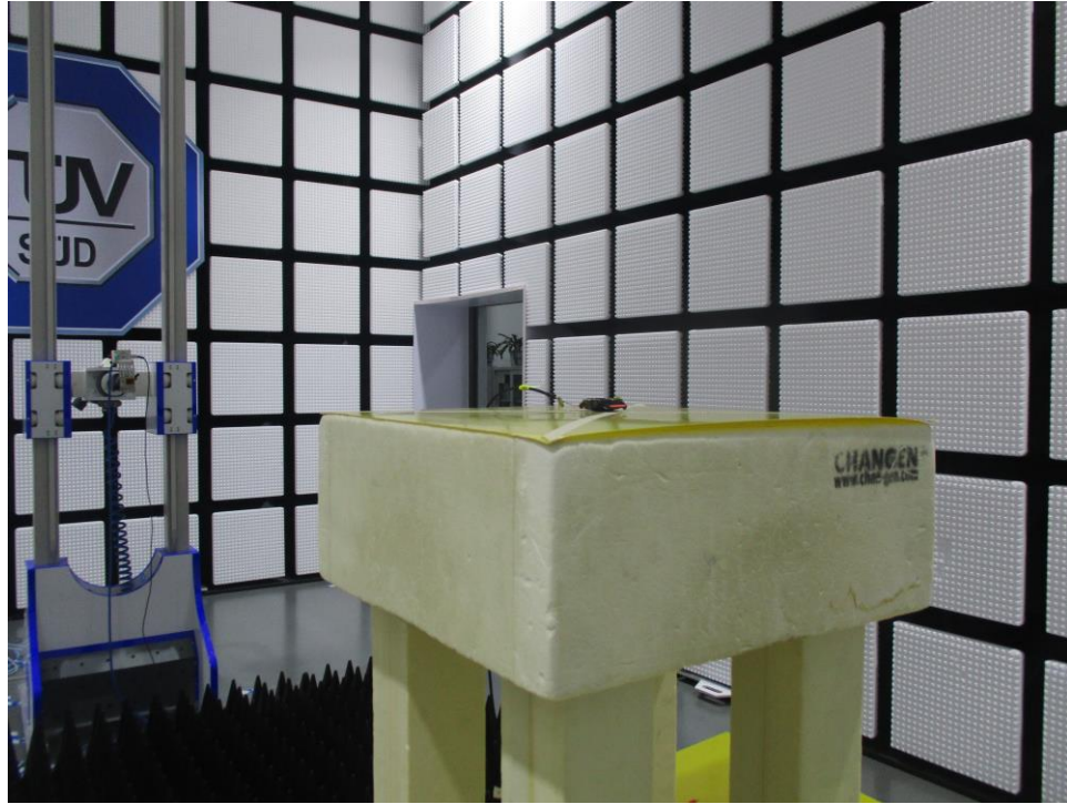
18G-40GHz Radiated spurious emission
