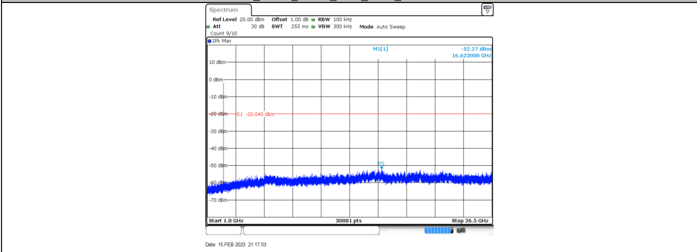
BLE_2MHz_BT5.0_Ant1_2480_0~Reference
