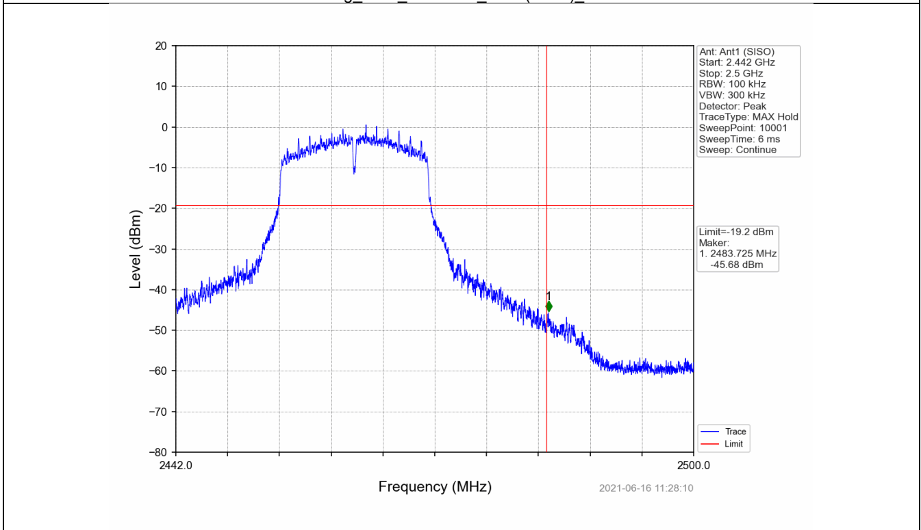
802.11g_HCH_2462MHz_Ant1 (SISO) NTN
