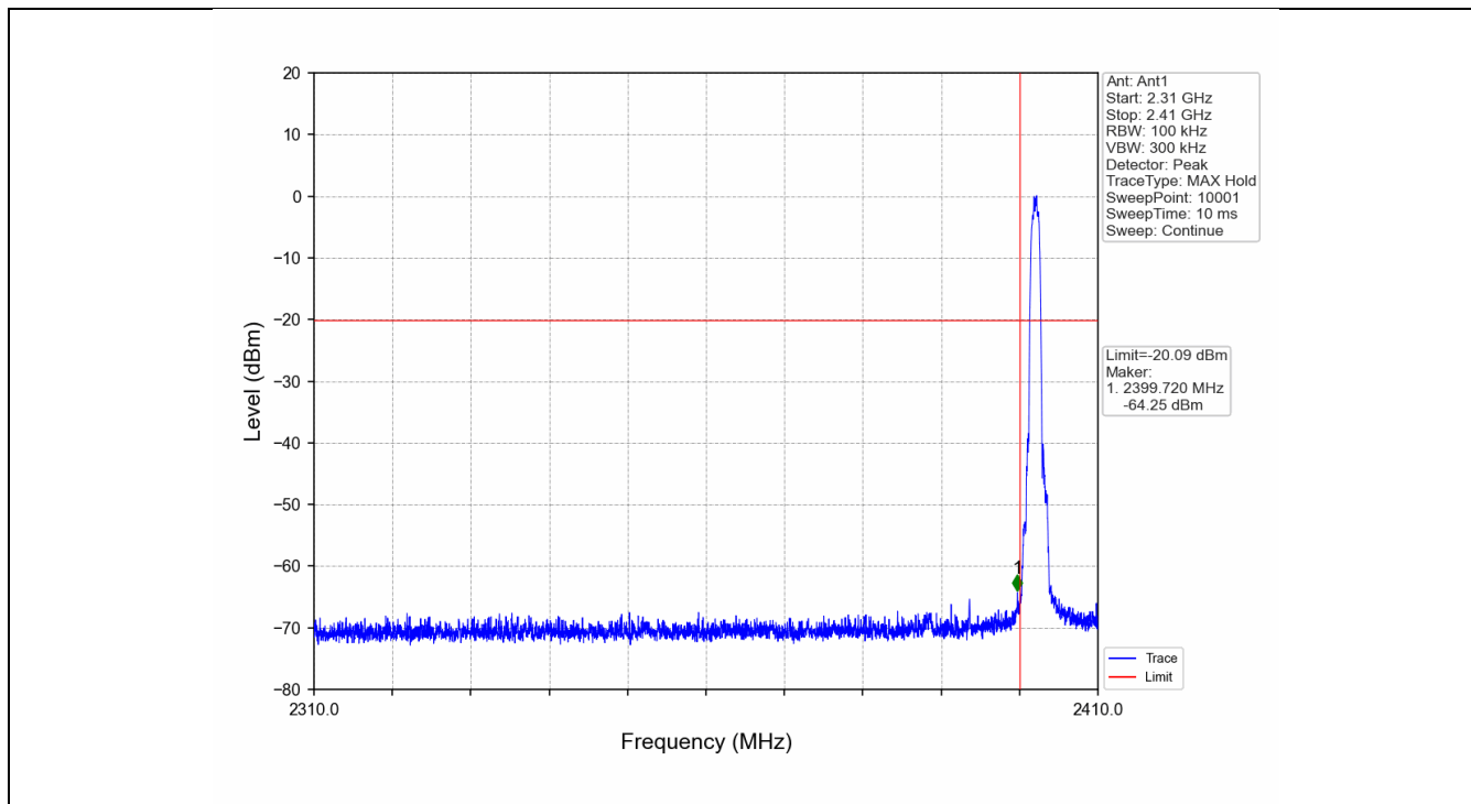
Pi/4DQPSK_2DH5_LCH_2402MHz_Ant1_NTNV
