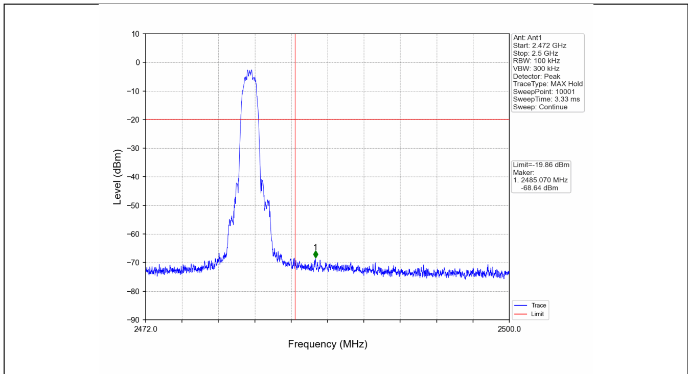
8DPSK_3DH5_HCH_2480MHz_Ant1_NTNV
