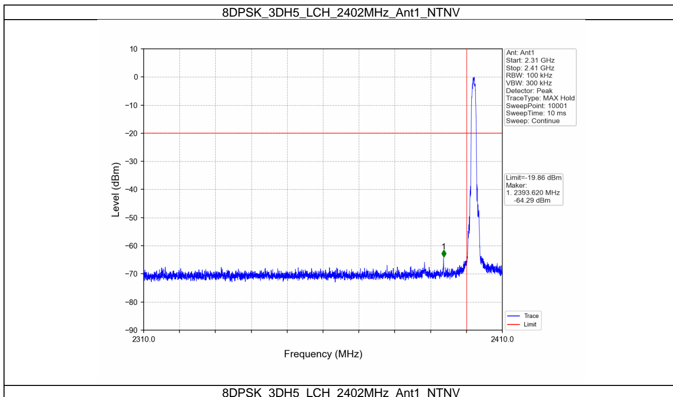
8DPSK_3DH5_LCH_2402MHz_Ant1_NTNV
