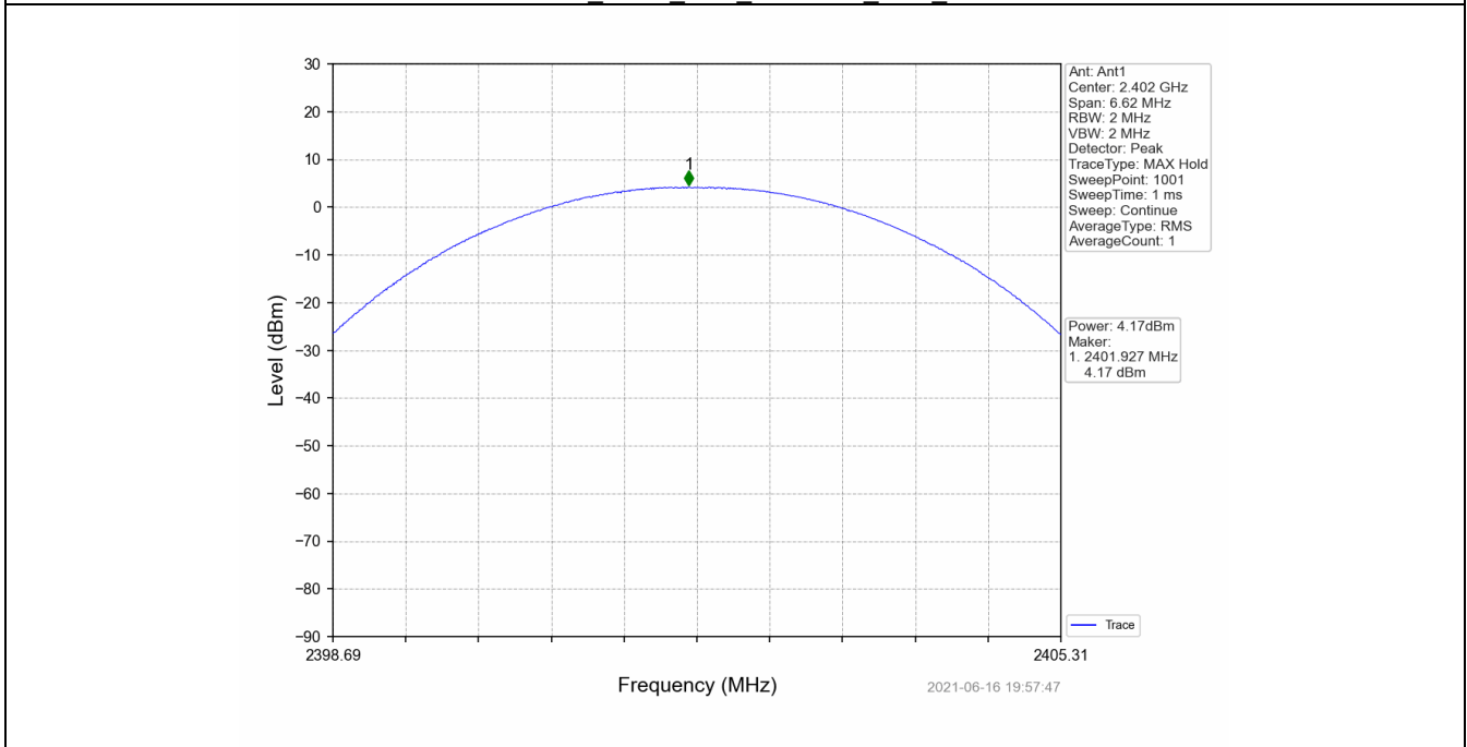
Pi/4DQPSK_2DH5_LCH_2402MHz_Ant1_NTNV
