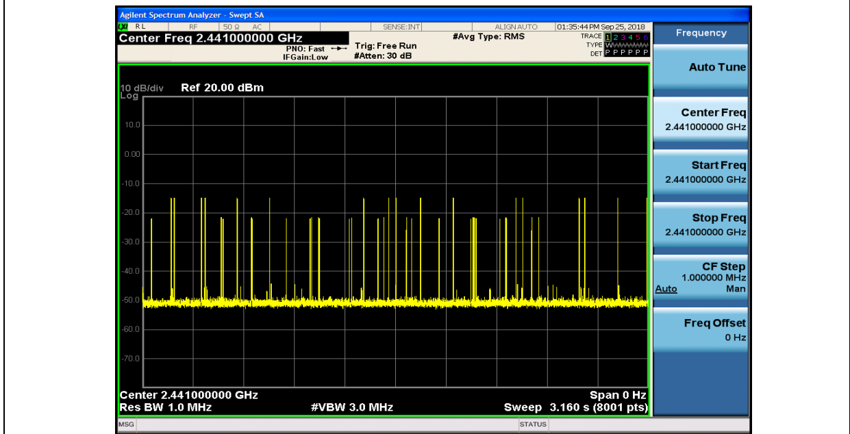
Dwell Time_3DH5_2441
