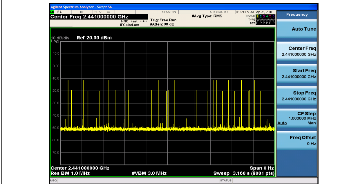
Dwell Time_3DH1_2441
