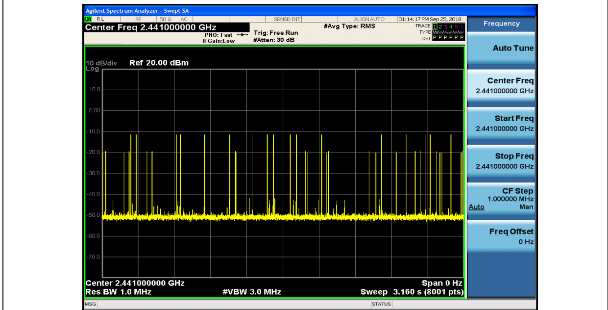
Dwell Time_DH5_2441
