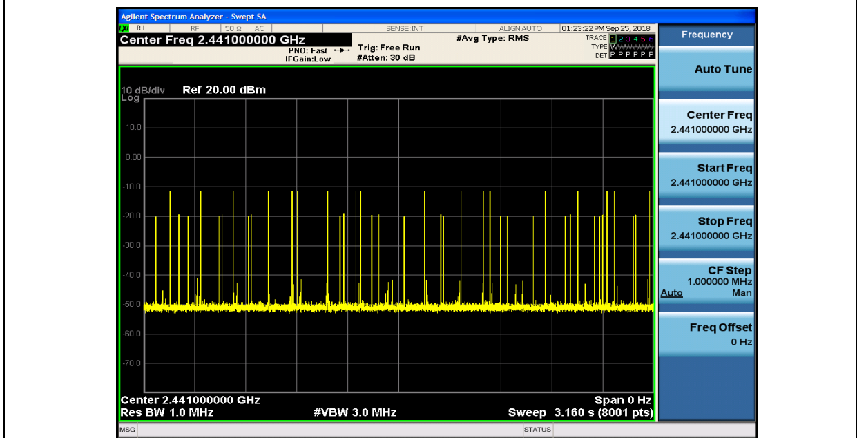
Dwell Time_2DH5_2441
