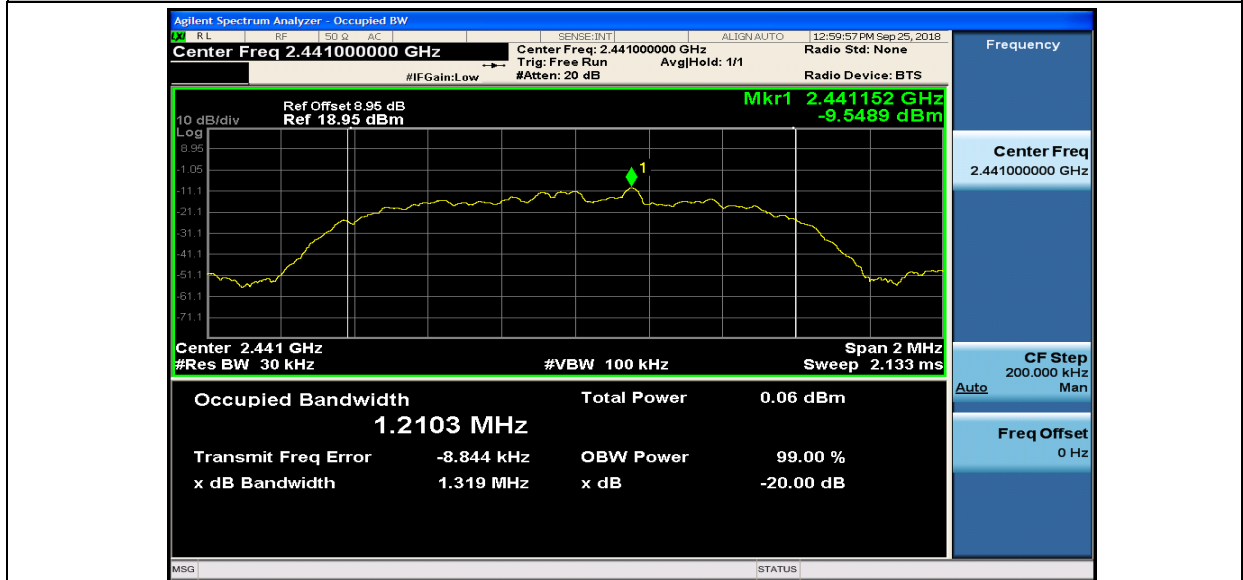
20 dB Bandwidth_3DH5_2480
