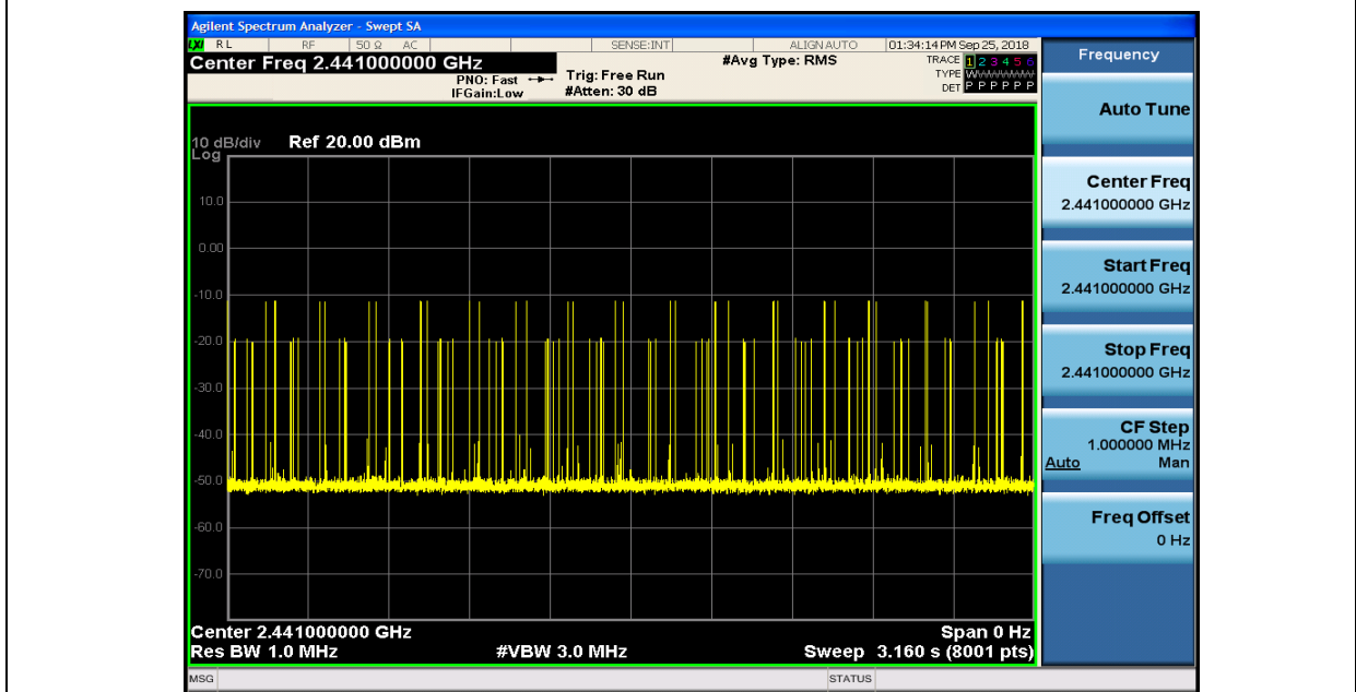
Dwell Time_3DH3_2441
