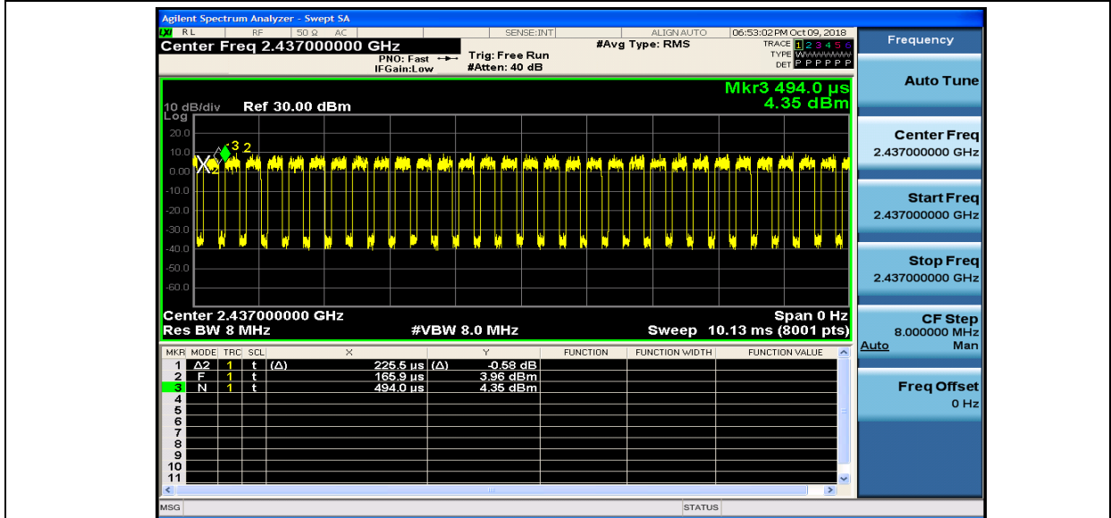
Duty Cycle_11N20SISO_2437_Ant4
