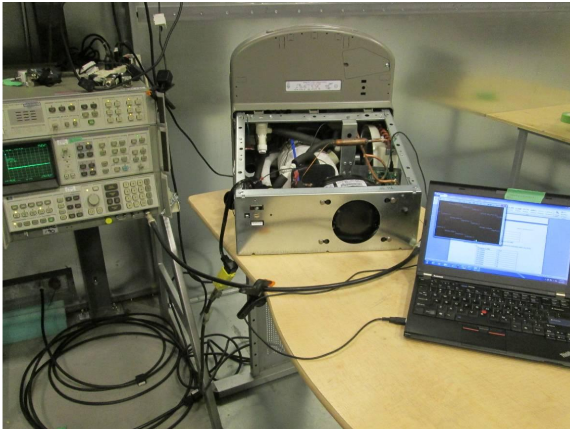
Photo 4. Conducted Measurements
