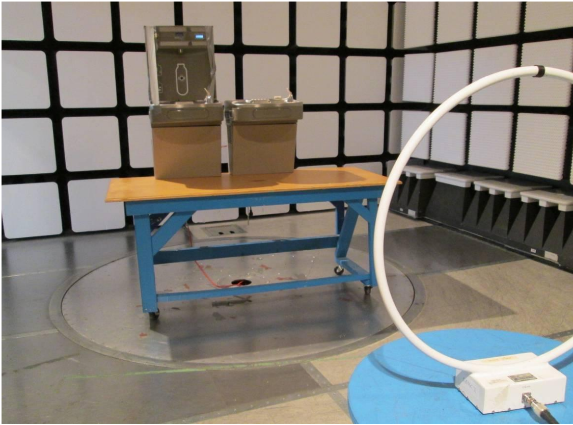
Photo 1. Radiated Emissions 1 Testing on unit with Alpha-numeric Display connected. Setup for unit with Graphic Display and RF testing are similar.
