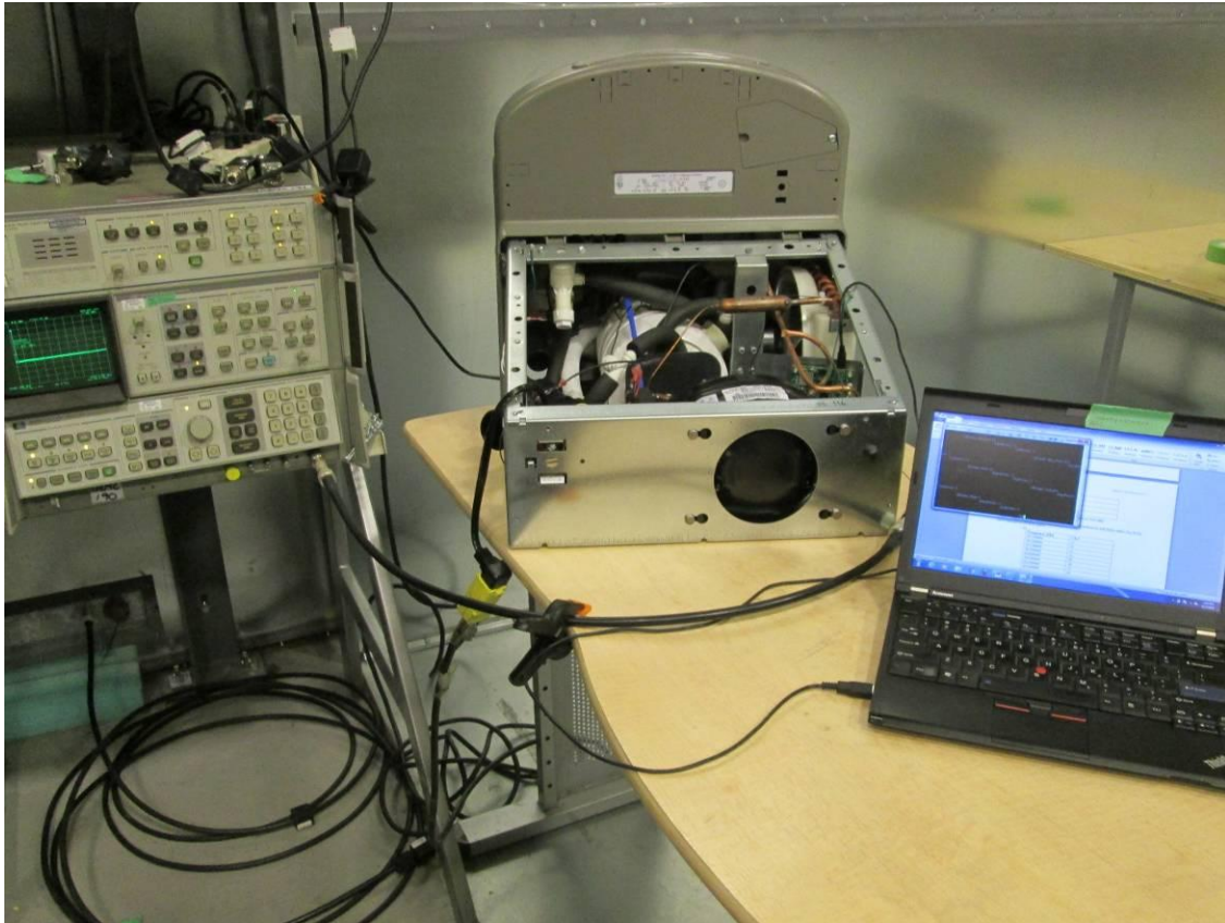
Photo 4. Conducted Measurements
