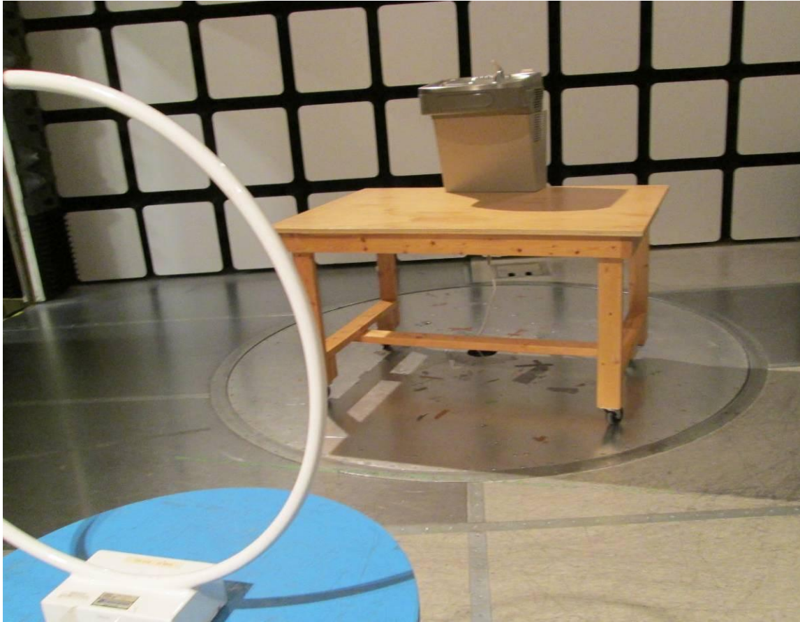
Photo 3. Radiated Emissions 3 Testing on RF board
