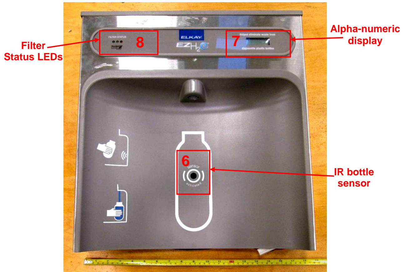
Photo 4. EUT – Exterior view, Part # 1 Alpha-numeric Display detached from fountain
