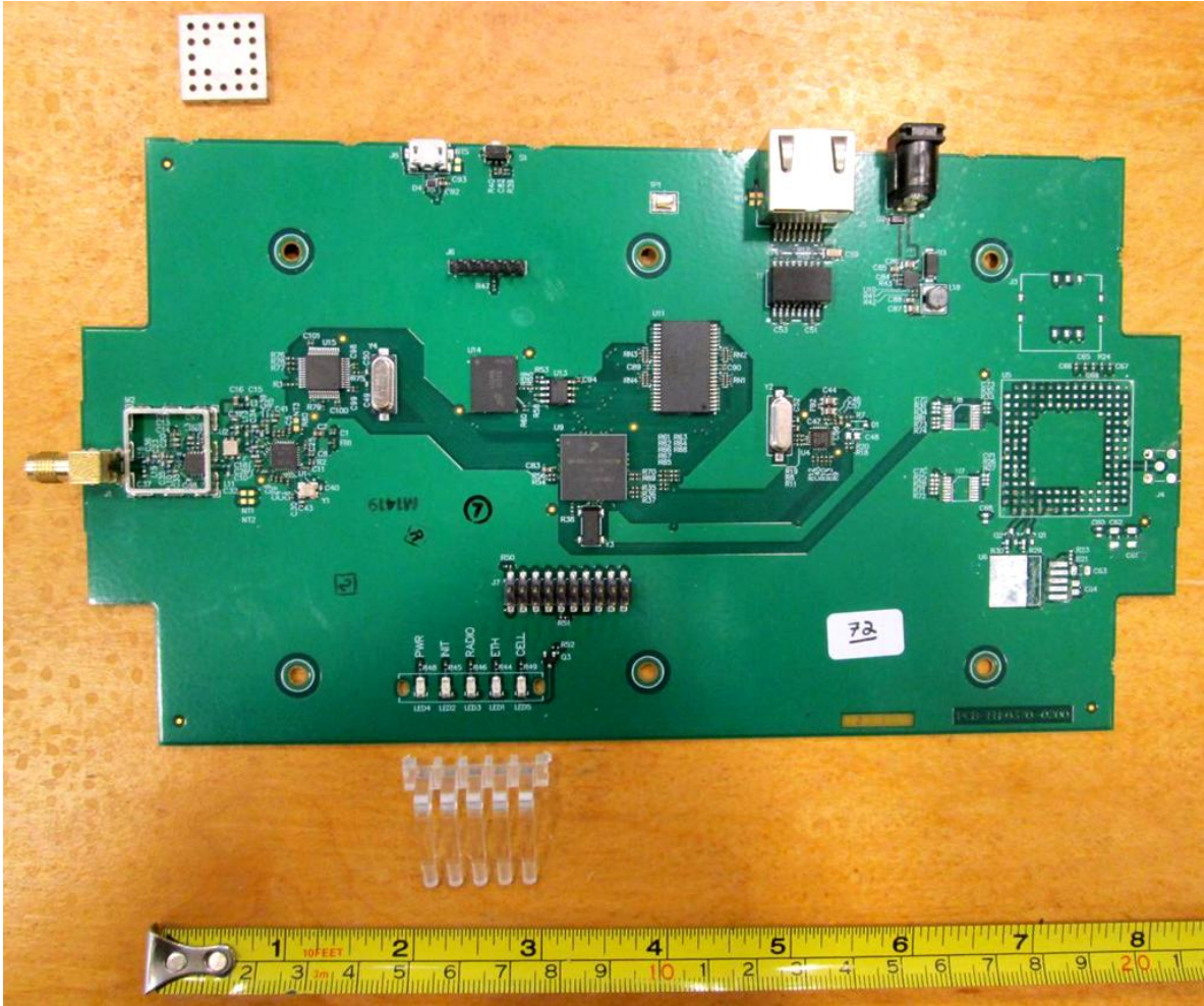
Photo 2. EUT – Internal view PCB, view 1, with shield removed
