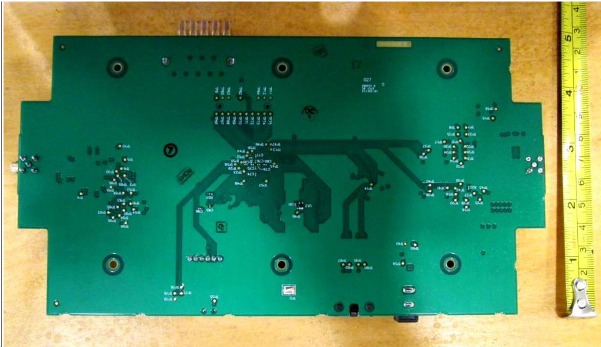
Photo 3. EUT – Internal view PCB, view 2
