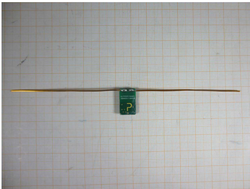
Photo 10: DiPol_STP-868 antenna
