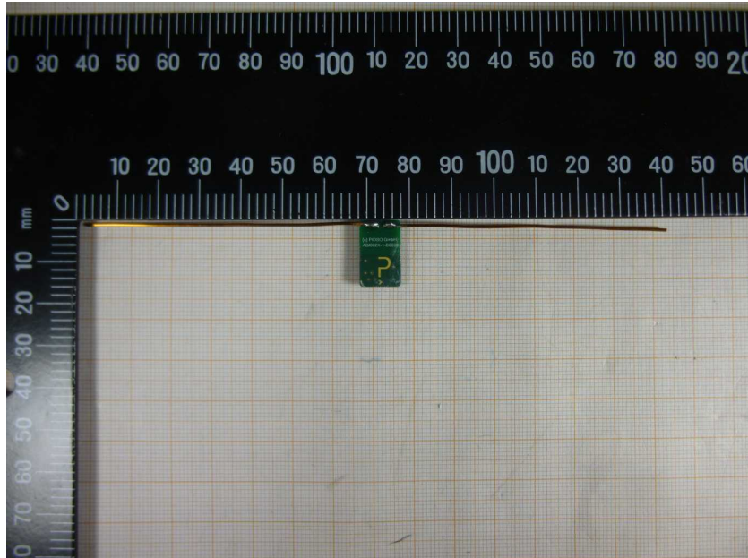
Photo 11: DiPol_STP-868 antenna
