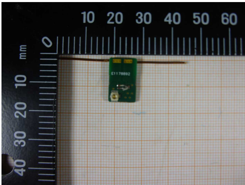
Photo 6: DiPol_STP-2G4 antenna
