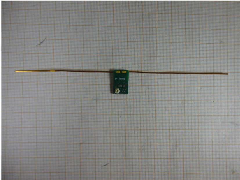
Photo 9: DiPol_STP-868 antenna
