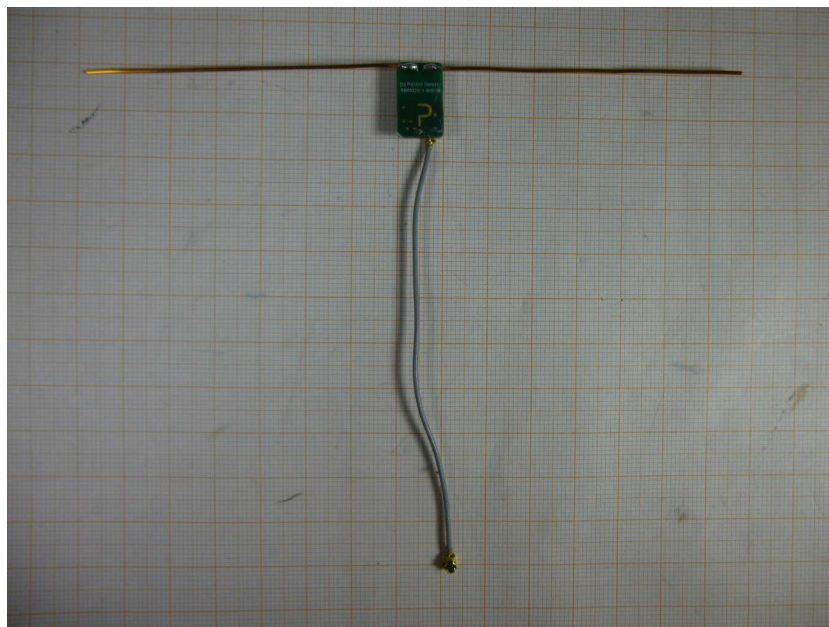
Photo 8: DiPol_STP-868 antenna with cable
