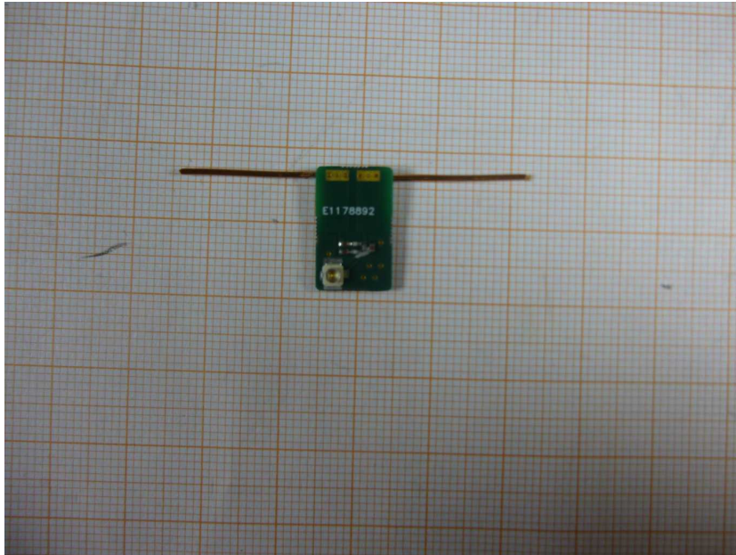
Photo 5: DiPol_STP-2G4 antenna
