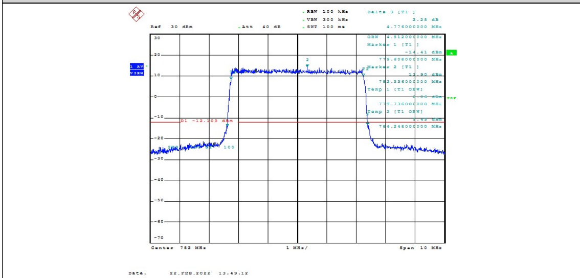
Band13-5MHz-QPSK-23230-25RB#0-4.512
