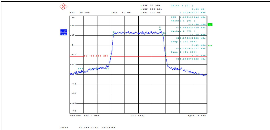
Band26-1.4MHz-QPSK-26797-6RB#0-1.096
