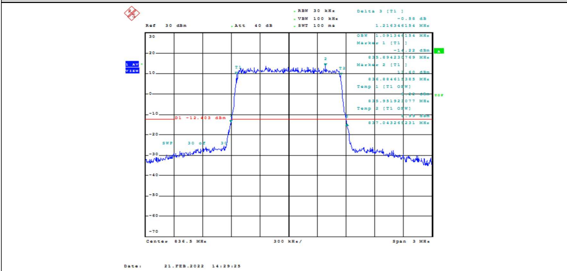
Band26-1.4MHz-16QAM-26915-6RB#0-1.091
