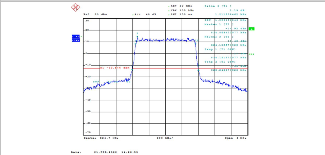
Band26-1.4MHz-16QAM-26797-6RB#0-1.096
