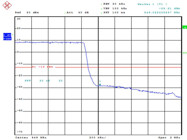
Band26-1.4MHz-16QAM-27033-1RB#5
