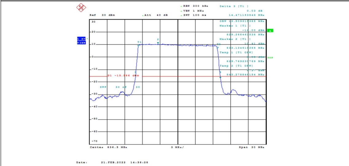
Band26-15MHz-QPSK-26915-75RB#0-13.51
