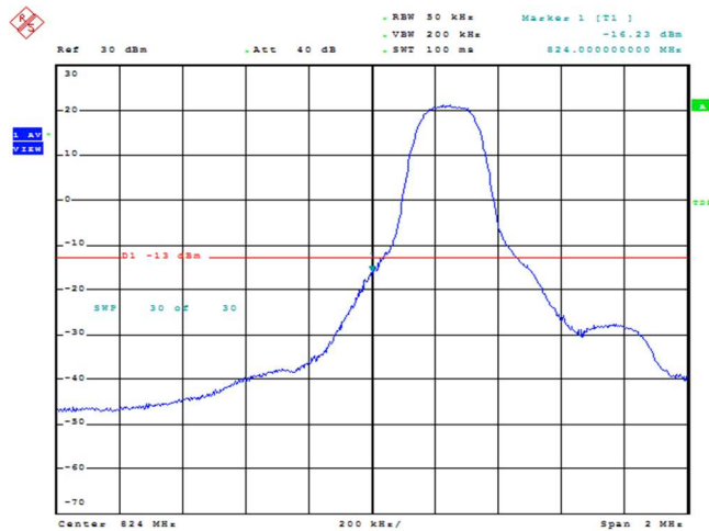
Band26-1.4MHz-16QAM-27033-6RB#0
