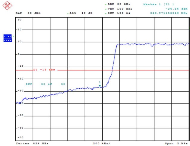
Band26-1.4MHz-16QAM-26797-1RB#5
