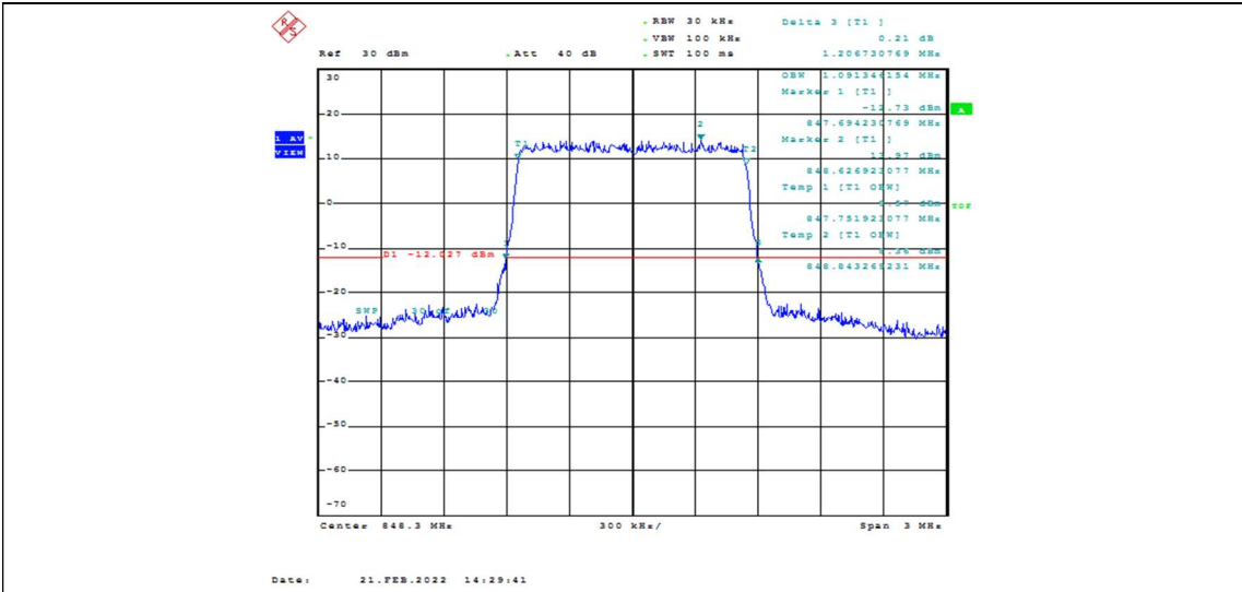
Band26-1.4MHz-QPSK-27033-6RB#0-1.091
