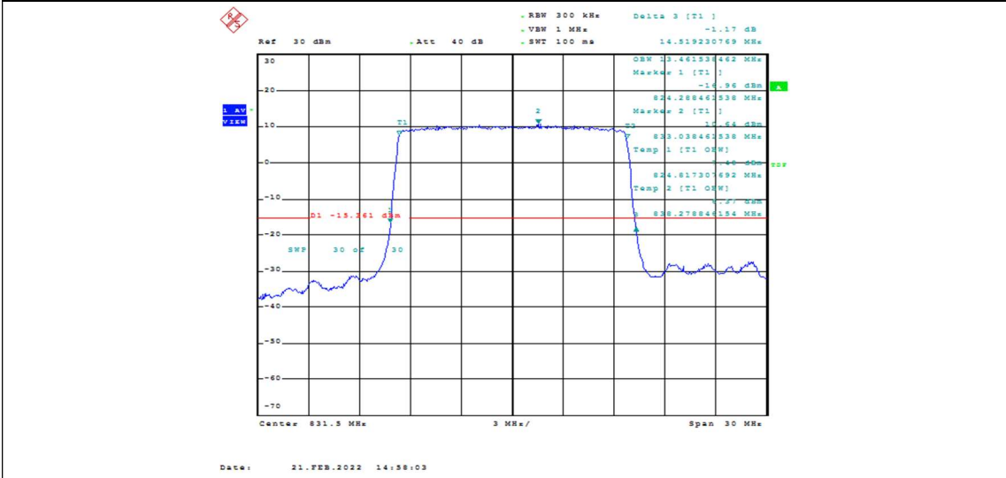
Band26-15MHz-QPSK-26865-75RB#0-13.462
