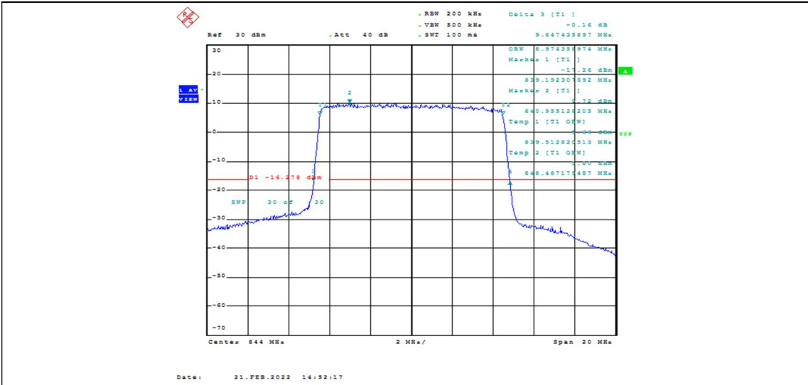
Band26-10MHz-16QAM-26990-50RB#0-8.974
