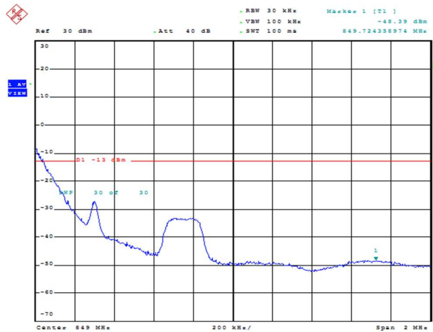
Band26-1.4MHz-16QAM-26797-6RB#0
