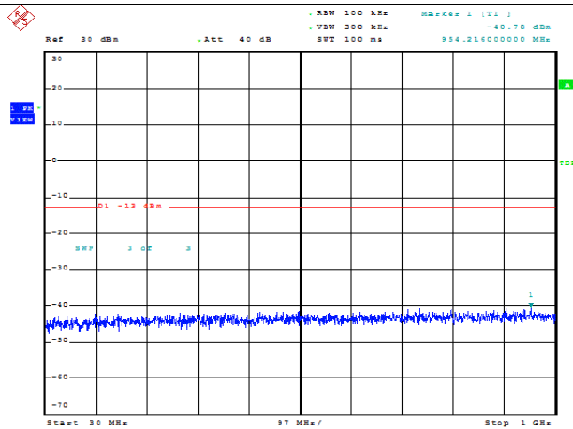
Band25-20MHz-QPSK-26590-1RB#0-Range1:30~1000MHz
