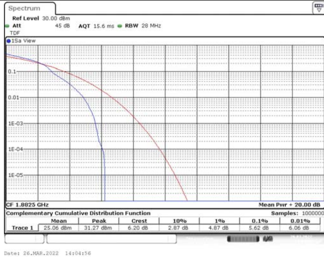
Band25-5MHz-16QAM-26365-1RB#0
