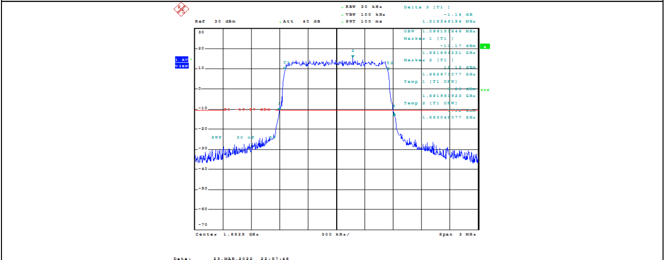
Band25-1.4MHz-QPSK-26365-6RB#0-1.096
