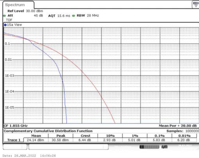
Band25-10MHz-16QAM-26090-1RB#0
